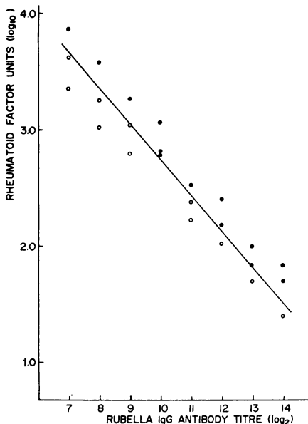
Fig. 2 Occurrence of false-positive rubella IgM antibody results correlated to rheumatoid factor levels and rubella IgG antibody titres. In the experiment, three sera were blended to obtain serum mixtures with different IgG titres and rheumatoid factor levels: (●) serum giving a false-positive rubella IgM antibody result; (○) serum giving a negative rubella IgM antibody result. The solid line represents the discriminant function ( z = x + 3.24y, z_0 = 18.9 ).
