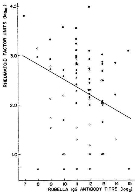
Fig. 1 Occurrence of false-positive rubella IgM antibody results correlated to rheumatoid factor levels and rubella IgG antibody titres of serum specimens from 61 patients with rheumatoid arthritis and 12 other patients without acute rubella infections: (●) serum giving a false-positive rubella IgM antibody result; (○) serum giving a negative rubella IgM antibody result. The solid line represents the discriminant function ( z = x + 6.51y, z_0 = 26.4 ).
