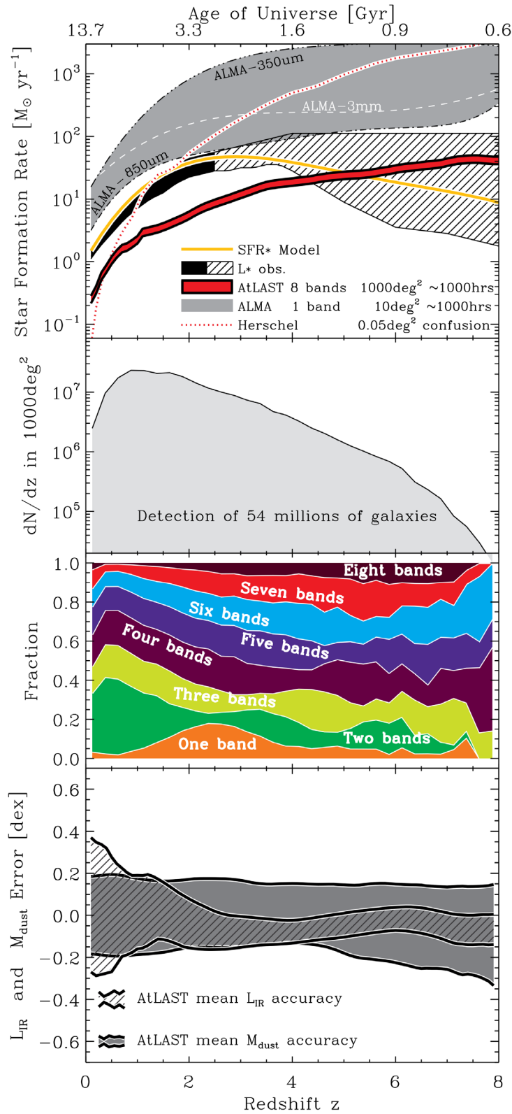
Figure 3. Exploring the parameter space of a 1000 deg 2 survey using 1000 hours of AtLAST observing time. Top panel: SFR vs. redshift survey limit. Second panel: dn/dz . The third panel shows the fraction of (mock) sources detected on 1, 2, 3, ..., or all 8 bands. The bottom panel shows the expected AtLAST accuracy in inferring L_{IR} and M_{dust} as a function of redshift (better than 25% and 50% at z > 2 , respectively), demonstrating why multi-band detections are important.
