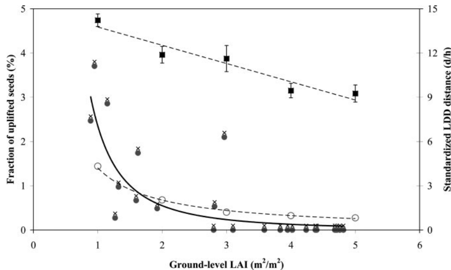
Fig. 3. The mean predicted distance traveled by uplifting seeds (filled squares), and the mean predicted (open circles) and observed (filled circles) uplifting probability, as a function of LAI. For generality, the dispersal distance ( d ) is standardized by the forest top canopy height ( h ), equal to 33 m in our site. The predicted values calculated by varying seed terminal velocity ( V_t ) from 0.5 to 2 m s -1 , release height ( H_r ) from 0.5 to 0.95 h , and u_* are taken from the overall Weibull function (Table 1 and Fig. 4; u_* > 0.5 m s -1 ). The observed values are calculated as the fraction of seeds collected from traps above the top canopy height, from the total number of seeds collected from tower traps, for each census period (typically 1–2 weeks) for which LAI data were available. The predicted dispersal distances of uplifted seeds is a strong linear function of LAI ( d/h = 15.00 - 1.24 \text{ LAI} ; R^2 = 0.92 , P_{(\text{slope}=0)} < 0.001 ; upper dashed line). The predicted uplifted probability is very accurately described by an inverse power law function of LAI ( d/h = 1.40 \text{ LAI}^{-1.05} ; R^2 = 0.99 , P_{(\text{slope}=0)} < 0.001 ; lower dashed line). The observed estimates of uplifting probability include many zero values; hence, the distribution is not amenable for power law or exponential regression. A small increment of 0.1, indicated by crosses, gives a fair fit for the inverse power ( d/h = 2.36 \text{ LAI}^{-2.10} ; R^2 = 0.76 , P_{(\text{slope}=0)} < 0.001 ; solid line). We note that the parameter values for this inverse power function are extremely sensitive to the size of the increment, whereas the coefficient of determination is rather stable. This suggests that the inverse power law describes the observed pattern fairly well but precludes any interpretation from these specific parameter values.
