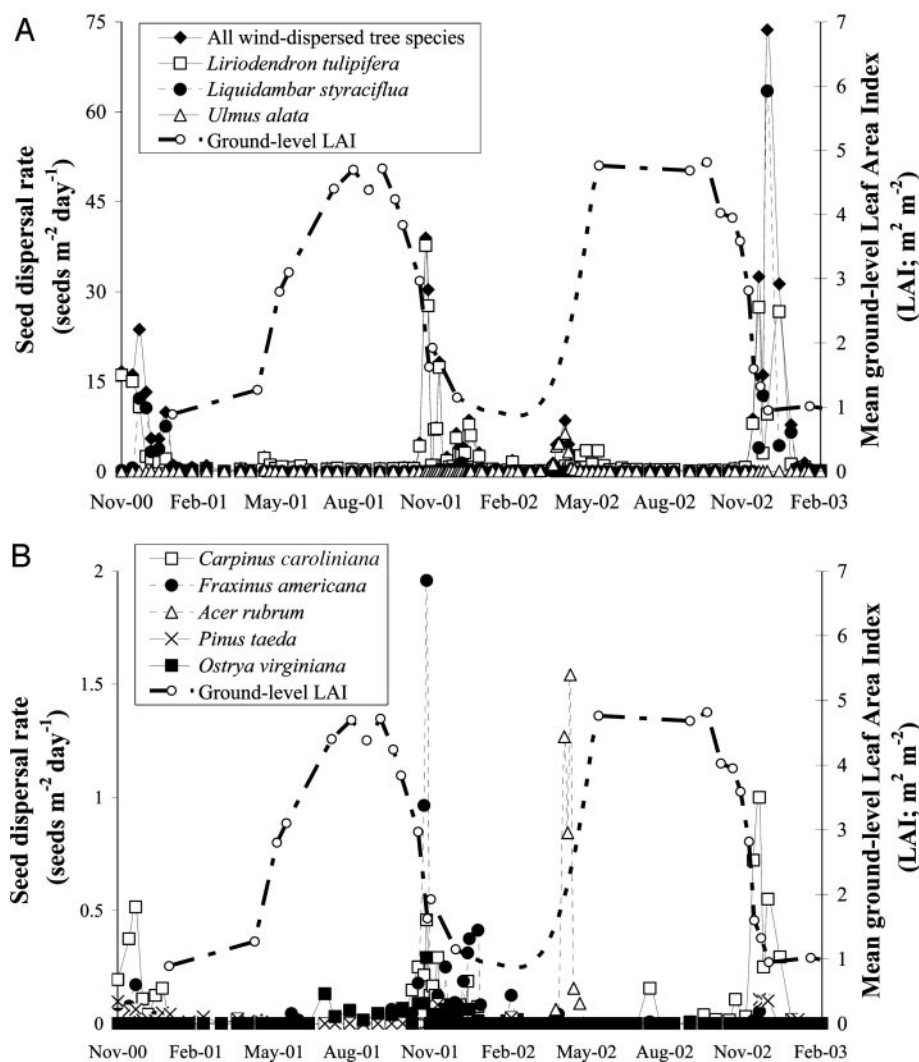
Fig. 1. Seasonal dynamics of seed dispersal and LAI observed near the meteorological tower at Duke Forest over 27 successive months. Note the difference in dispersal rates between species that were common (A) and rare (B) in the seed traps. The seasonal variation in LAI is shown in both panels for reference. LAI measurements were missing for the period between 2 December 2001 and 18 May 2002; the line drawn between these two points follows a second-order polynomial fitted for LAI data collected during the corresponding period in the previous and the subsequent (not shown) years.
