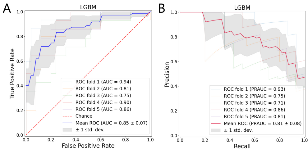
Fig. 3. The training performance of the five cytokine features derived LGBM modelling based on Training1 of division 1. (A). The mean AUC curve is shown in blue. The light gray shade shows the standard deviation stemming from the five-fold-cross validation results. (B). The PRAUC mean is shown in red. The light gray shade shows the standard deviation stemming from the five-fold-cross validation results. AUC: Area Under the Curve, PRAUC: Precision Recall Area Under the Curve.
