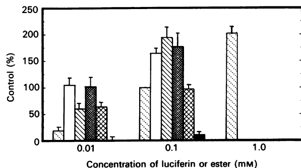
Fig. 4. Peak luminescent value obtained with intact cos cells after addition of luciferin or the luciferin esters
