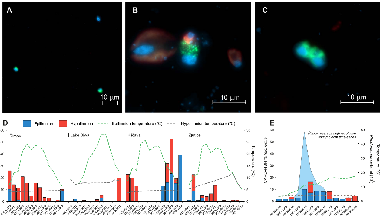
Figure 3. CARD-FISH images of Telonemia targeted by the probe Telo-1250. Green: CARD-FISH probe, blue: DAPI, red: autofluorescence (A) from Lake Cinciš (20 m) (B) from Řimov reservoir (0.5 m), Telonemia ingesting a Rhodomonas . A larger Cryptomonas and smaller Rhodomonas are also seen left and right, respectively, and (C) a dividing Telonemia cell from Breiter Luzin hypolimnion (50 m). All scale bars are 10 \mu\text{m} , panel (A) is in magnification 40X, and panels (B) and (C) are in 100X magnification. (D) Four annual time-series from Řimov reservoir, Lake Biwa, Kličava reservoir and Žlutice reservoir showing relative abundances of Telonemia (using CARD-FISH) in epilimnion and hypolimnion. Temperatures are shown as green (epilimnion) and gray-dotted (hypolimnion) lines. (E) Relative abundances of Telonemia in epilimnion and hypolimnion during a high-resolution sampling of a spring phytoplankton bloom in Řimov reservoir. Counts of the most abundant Cryptophyte ( Rhodomonas ) are shown as a blue background and temperatures as lines.
