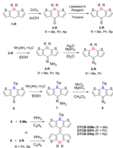
Scheme 1 Synthetic route of boron- and silicon-containing BAEs via the Barton–Kelllogg reaction.
