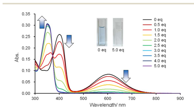
Fig. 7 Absorption data for titrations of DTCB-SiPh with TBACN aliquots in toluene at the concentration of 10 \mu\text{mol L}^{-1} .
