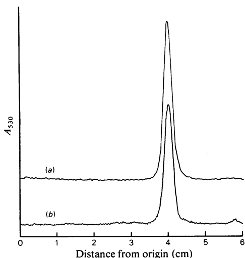
Fig. 4. Scan of an autoradiograph of sodium dodecyl sulphate/polyacrylamide-gel electrophoresis of (a) proteins of skeletal-muscle mitochondria incubated for 20 min with 0.2 mM-[ ^{32} P]P i (575 d.p.m./pmol)/5 mM-2-oxoglutarate/0.5 mM-L-malate and (b) [ ^{32} P]phosphorylated pig heart PDH complex
