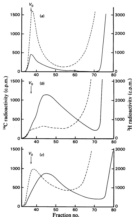
Fig. 1. Elongation of metabolically labelled [ ^3\text{H} ]hyaluronate by UDP-GINAc and UDP-[ ^{14}\text{C} ]GlcA in vitro . The Figure shows gel filtration on Sephacryl S-1000 of samples (a) without hyaluronidase treatment, (b) with hyaluronidase treatment of intact cells, and (c) a mixture of hyaluronidase-treated and untreated cells. Details were described in the Materials and methods section. -----, ^3\text{H} radioactivity; —, ^{14}\text{C} radioactivity. Low-molecular-weight fractions have been omitted for simplicity.
