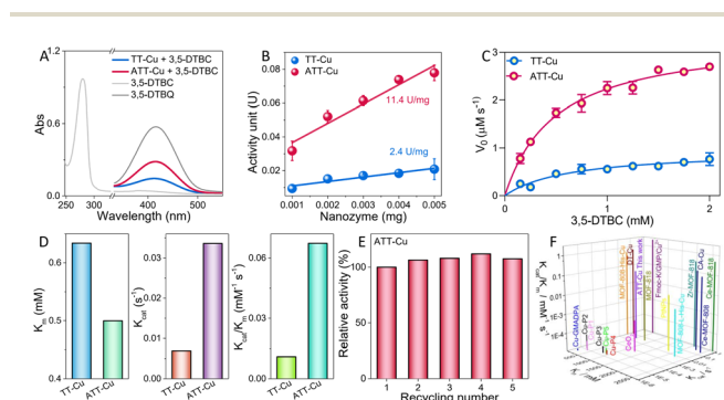
Fig. 4 Evaluation of CO-like activities of ATT-Cu and TT-Cu. (A) UV-vis spectra of 3,5-DTBC, 3,5-DTBQ and nanozyme-catalyzed oxidation of 3,5-DTBC in air-saturated PBS (pH = 8)/ \text{CH}_3\text{CN} solution; (B) specific activities; (C) Michaelis–Menten curves; (D) kinetic parameters ( K_m , K_{\text{cat}} and K_{\text{cat}}/K_m ); (E) recyclability; (F) comparison of the kinetic parameters ( K_m , K_{\text{cat}} and K_{\text{cat}}/K_m ) of ATT-Cu with reported CO-like artificial enzymes.
