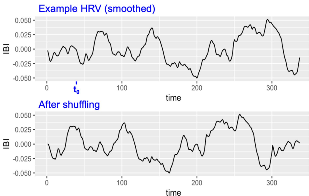
Fig. 5. Example IBI time series. Top pane: Original normalized smoothed values. Bottom pane: Shifted values after cyclic rotation using randomly chosen t_0 .
