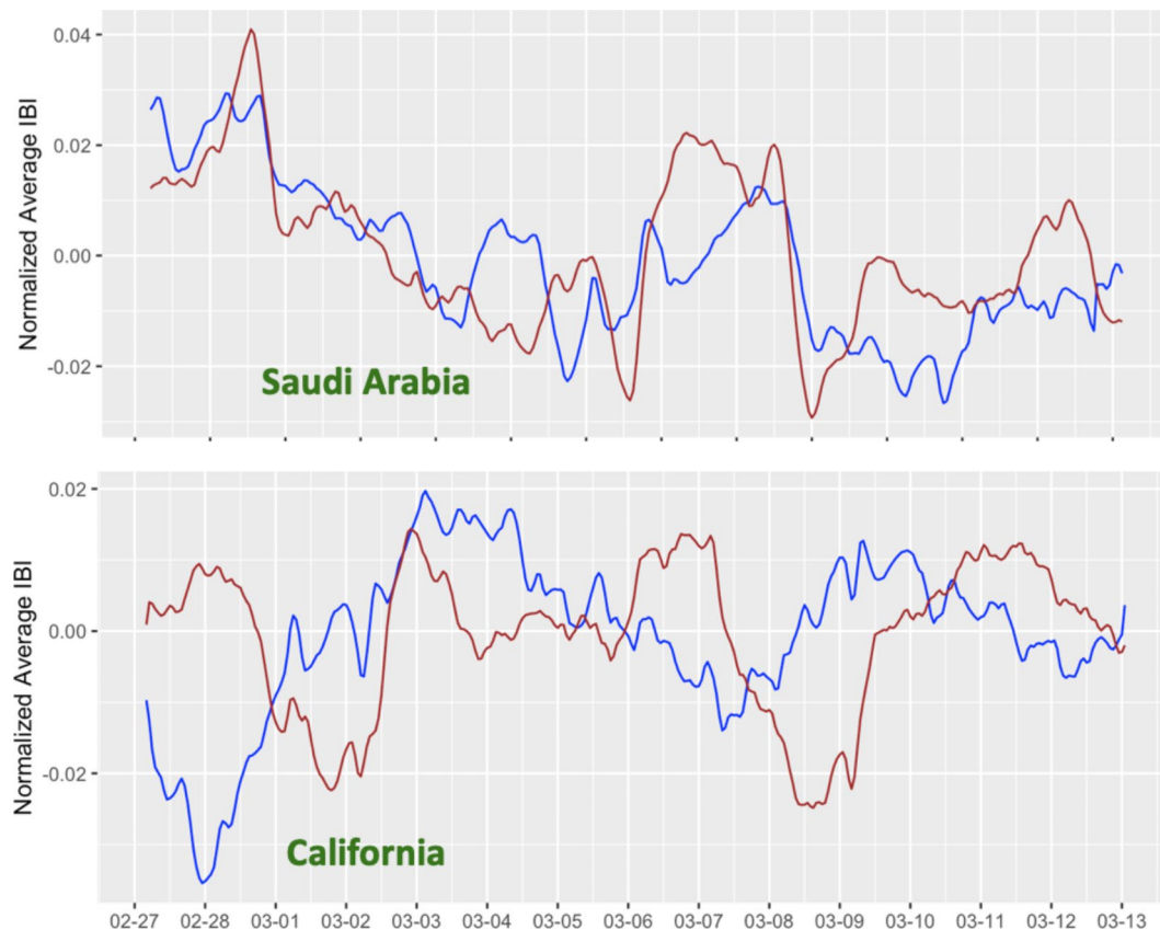
Fig. 3. Typical split half examples in two of the regions. In the top pane, when the Saudi Arabia group is split into two groups (blue and brown curves), the normalized average IBI of the groups are seen to be similar, with high correlation. In contrast, in the bottom pane, when the California group is split into two, the IBI's are seen to be different, with low correlation.
