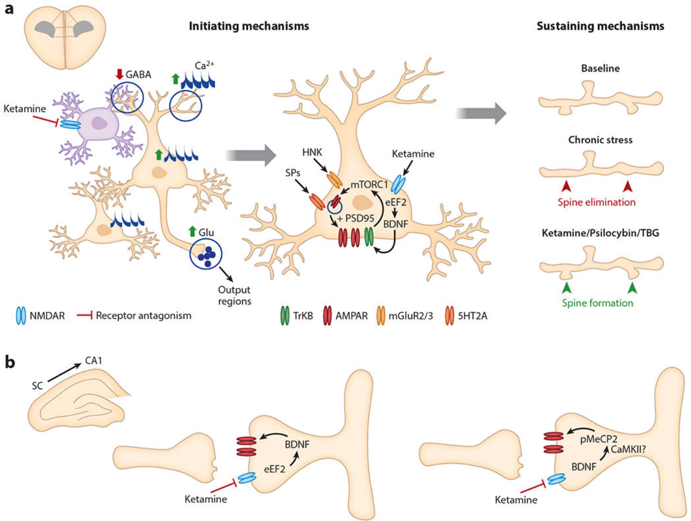
Figure 2. The initiating and sustaining mechanisms of rapid-acting antidepressants. (a) In the mPFC, ketamine acts to elevate glutamatergic tone of excitatory pyramidal neurons ( tan ), potentially through disinhibitory mechanisms involving tonically firing interneurons ( purple ). Ketamine leads to enhanced somatic and spine Ca^{2+} transients in layer 2/3 pyramidal cells within 1 h and increases multicellular ensemble activity within 3 h of administration ( left ). Ketamine, its metabolite HNK, and SPs each increase neurotrophic signaling and AMPAR insertion in mPFC excitatory neurons. The sustained antidepressant effects of ketamine and psychedelics involve targeted dendritic spinogenesis on excitatory projection neurons ( right ). Ketamine-induced spine formation is detected 12 h after administration and follows circuit reorganization. (b) In hippocampal SC to CA1 synapses, ketamine rapidly enhances BDNF release and increases postsynaptic glutamatergic transmission ( left ) while a sustained effect involves the delayed increase in pMeCP2 through a BDNF-dependent mechanism ( right ). Abbreviations: 5HT2A, 5-hydroxy-tryptamine receptor 2A; AMPAR, \alpha -amino-3-hydroxy-5-methyl-4-isoxazole propionic acid receptor; BDNF, brain-derived neurotrophic factor; Ca^{2+} , calcium; CaMKII, calcium-calmodulin kinase II; eEF2, eukaryotic elongation factor 2; GABA, \gamma -aminobutyric acid; Glu, glutamate; HNK, hydroxynorketamine; mGluR2/3,
