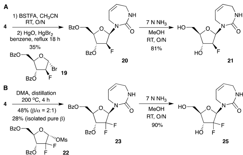
Scheme 5 Synthesis of fluorinated diazepinone nucleosides by direct glycosylation.
