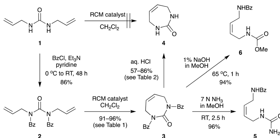
Scheme 2 Improved 3-step synthesis of 1,3-diazepinone by ring-closing metathesis.
