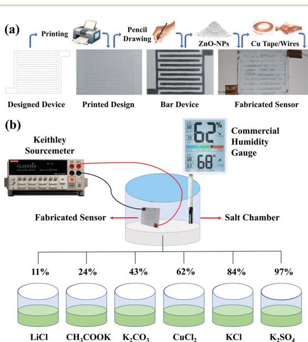
Fig. 1 (a) Digital photographs and illustrations showing the fabrication of the G/ZnO-NP-based humidity sensor. (b) Sensing setup for the humidity sensor.
