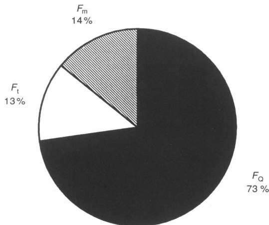
Figure 3. Factors limiting maximal oxygen consumption after bed rest
