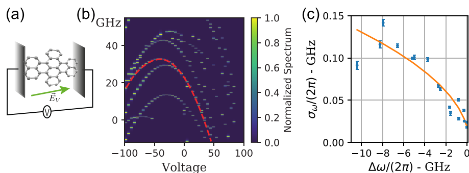
Figure 3. Stark shift and SD (a) cartoon picture of the specific configuration. We perform the spectral measurements on a DBT molecule embedded between two electrodes at fixed voltage difference generating a tunable in-plane electric field in the direction of the principal polarization axis defined by \alpha_{xx} . (b) Typical measurement of the excitation spectra (color coded along the y axis of the figure) as a function of the applied voltage on the electrodes. Each parabola can be associated with a different molecule. The measurements are obtained with a scan speed of 0.5 GHz/s. At this scanning speed the observed line is broadened by the fast components of SD. (c) Measured SD as a function of the frequency shift extracted from the data highlighted by the red dashed line in (b); the values of \sigma_\omega are extracted by fitting each fixed voltage spectrum with a Voigt profile. The orange line corresponds to the best fit of the square-root dependence of SD against the shift predicted in eq 3.
