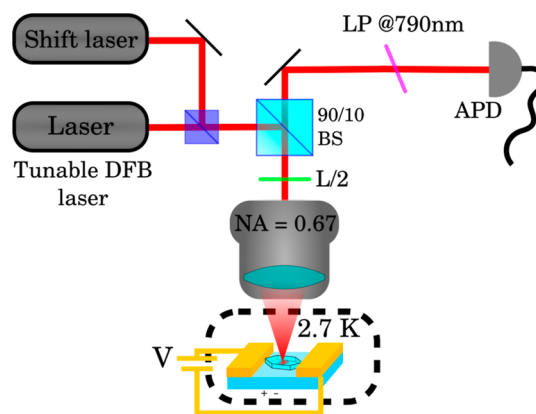
Figure 6. Optical setup. Molecules are excited and observed in a confocal microscope setup whose main elements are schematically shown here. BS stands for beam splitter, L/2 for half-wave plate, LP for long-pass filter, and APD for avalanche photodiode.
