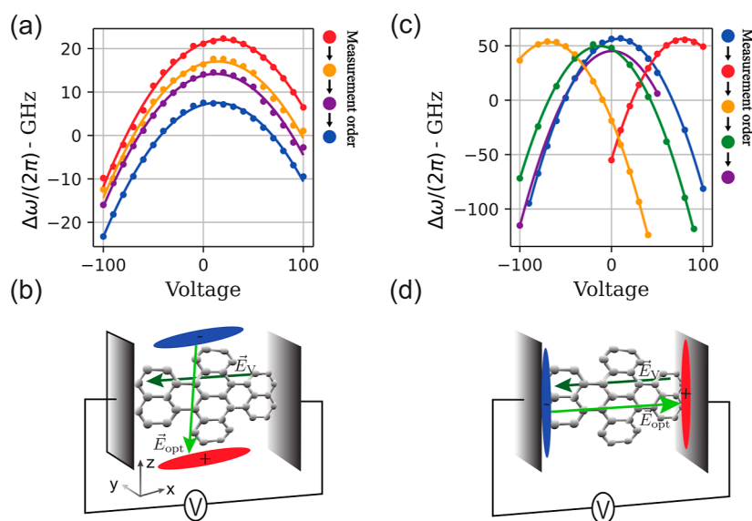
Figure 4. OSS and EGOSS. (a) Measured ZPL frequency shift \Delta\omega_{ZPL}/(2\pi) after subsequent OSS runs are plotted as colored dots. Solid lines represent the best fit to the data with parabolic functions. The experimental configuration is sketched in panel (b). Applying the optical shift results in an accumulation of charges along the z axis that gives rise to an electric field along the secondary polarizability axis of the DBT molecule; as a second step, an in-plane electric field along the x axis is applied through the electrodes, varying the voltage V . (c) Measured ZPL frequency shift \Delta\omega_{ZPL}/(2\pi) after subsequent EGOSS runs are plotted as colored dots. Solid lines represent the best fit to the data with parabolic functions. The experimental configuration is sketched in panel (d). In this case, fixed bias voltages impose a preferential direction for the excited charges to move, accumulating them in the direction of the electrodes-applied field. This results in an effective screening of the in-plane electric field between the electrodes and hence in an electric field offset in the Stark-parabola. All OSS and EGOSS cycles have been performed with 100 \mu\text{W} pump power. Applied voltages and exposure times are reported in the legends next to the plots.
