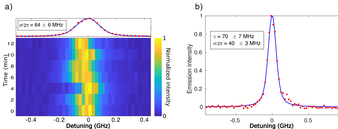
Figure 2. Excitation spectroscopy and SD. The excitation spectrum from a DBT emitter, obtained by recording the red-shifted fluorescence signal (red dots) as a function of the excitation laser frequency, is fitted by a Voigt profile (blue solid lines). The homogeneous ( \gamma ) and inhomogeneous ( \sigma ) broadening components can be extracted from the fits. Here, each overall swipe is obtained at a scan speed of 0.5 GHz/s. (a) Each line corresponds to an excitation spectrum plotted in color scale. The total measurement time for the repeated swipes amounts to 12 min. The integrated signal is plotted in the top panel. (b) A single snapshot is shown where the lower \sigma component confirms that the SD depends on the observation time.
