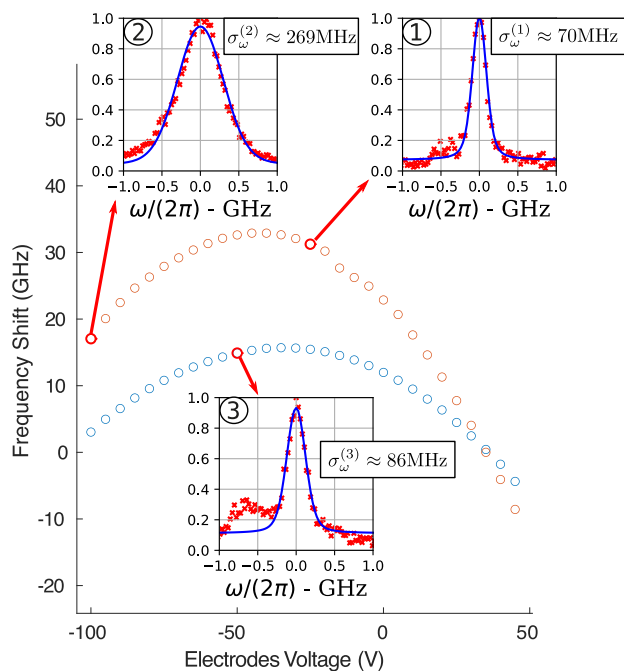
Figure 5. Effect of electric field control on SD. The parabolas are obtained by monitoring the frequency of emission of a molecule during a scan over the electrode voltage. The orange dots are measured before any optical shift while the blue ones after a combined shift that allowed for the creation of a local field in the z direction. In correspondence to the red highlighted points, we measured SD by repeating excitation spectroscopy measurements. The integrated signal is presented in the insets. A Voigt profile fit on each of the integrated signals allowed for the isolation of the Gaussian component of the broadening associated with SD.
