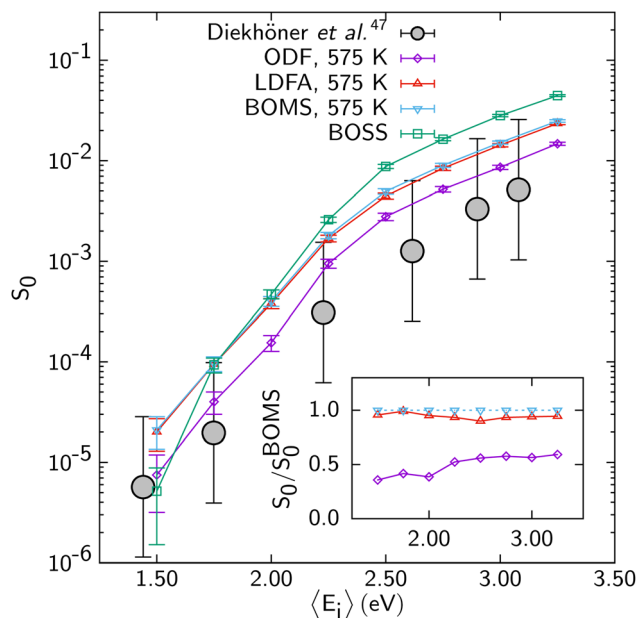
Fig. 5 S_0 computed for N_2 + Ru(0001) with MDEF and the RPBE DF using the Born–Oppenheimer static surface (BOSS) model, 70 the Born–Oppenheimer moving surface (BOMS) model, 70 the Born–Oppenheimer moving surface (NBOMS) model with the LDFA and the ODF approximations 69 are shown as a function of E_i . Experimental results are also shown. Figure taken from ref. 69 ( https://pubs.acs.org/doi/10.1021/acs.jpcllett.9b00523 ). Further permission requests to be directed to the ACS.
