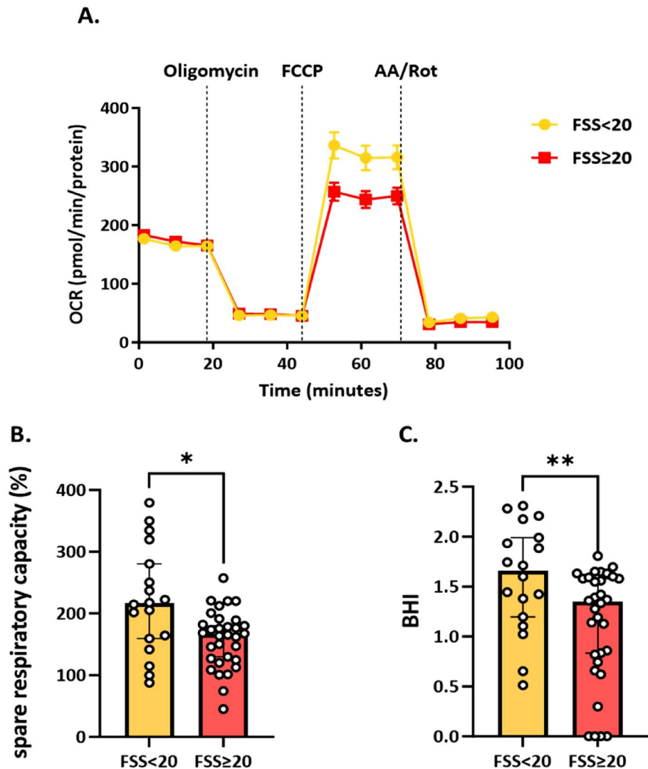
Fig. 2. Evaluation of mitochondrial functionality in peripheral blood mononuclear cells (PBMC) of patients with fibromyalgia syndrome and a FSS < 20 ( n = 18 ) and in the group with FSS \geq 20 ( n = 32 ). Panel A shows the oxygen consumption rate (OCR) measured through the Seahorse XF Cell Mito Stress Test. Panel B indicates the spare respiratory capacity (as expressed in %) and Panel C the distribution of BHI. Orange bars represent the group with FSS < 20 and red bars represent the FSS \geq 20 group. Results are expressed as median (Q1, Q3). Differences between groups were by Mann–Whitney U test, * p < 0.05 ; ** p < 0.01 . AA Antimycin A; BHI, Bioenergetic Health Index; FCCP Carbonyl cyanide-4 (trifluoromethoxy) phenylhydrazone; FSS, Fibromyalgia Severity Score; OCR, Oxygen Consumption Rate; PBMCs, peripheral blood mononuclear cells; Rot, rotenone.
