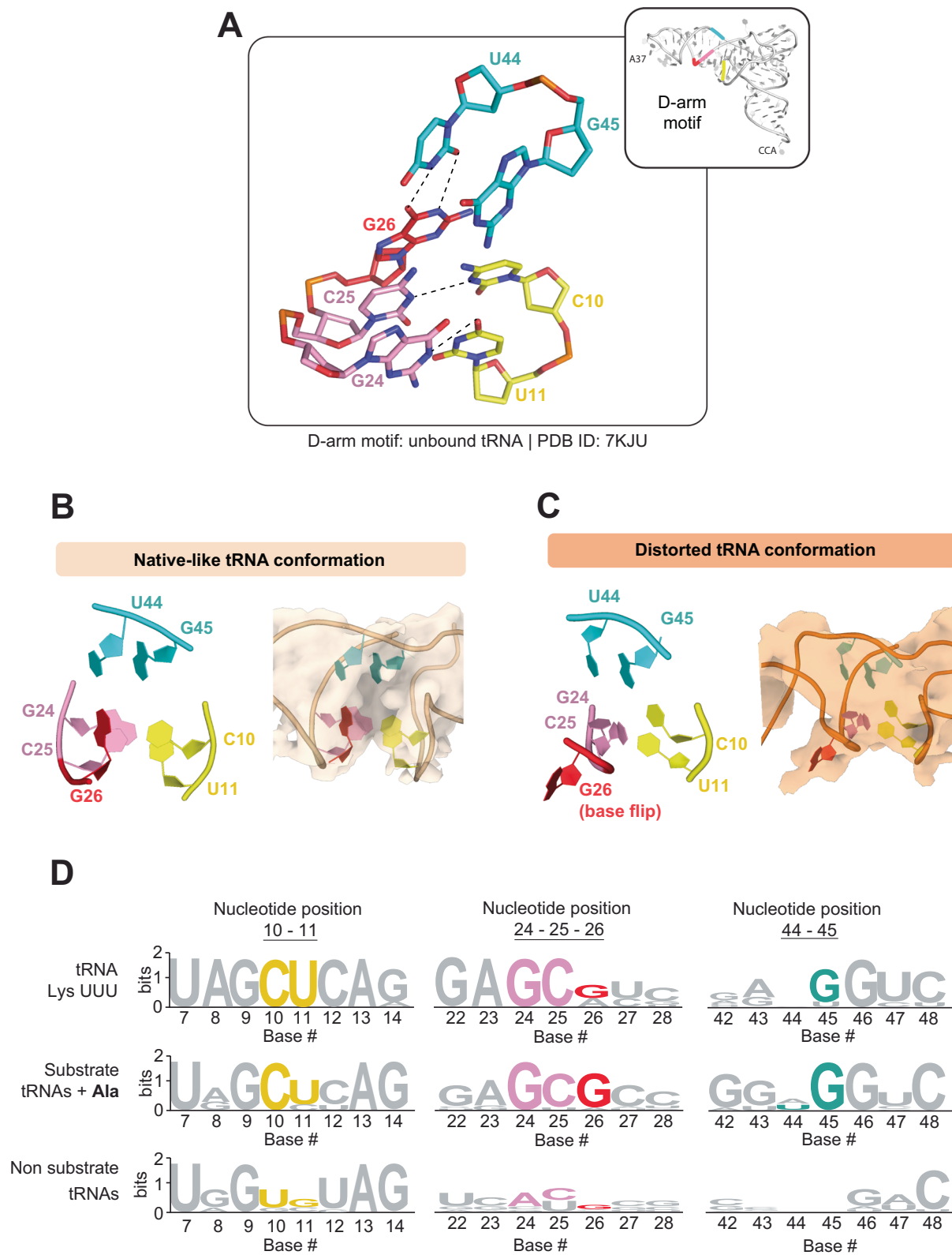
Fig. 3 | G26 resides within a network of nucleotides conserved in KEOPS substrate tRNAs. A Stick representation of the D-arm motif network as observed in the crystal structure of M. jannaschii tRNA Lys (PDB 7KJU). G26 forms hydrogen bonds with U44, and base stacking interactions with C25 and G24. G24 and C25 base pair with U11 and C10, which stack with G45. (right) Cartoon representation of tRNA structure showing the location of the D-arm nucleotides according to their coloring scheme shown in the left. B, C Atomic models (left) and cryo-EM density volumes
