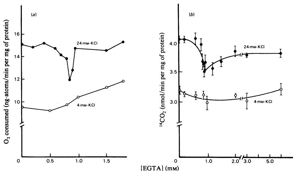
Fig. 4. The effect of EGTA on the rate of O 2 consumption (a) and [1- 14 C]pyruvate decarboxylation (b)
