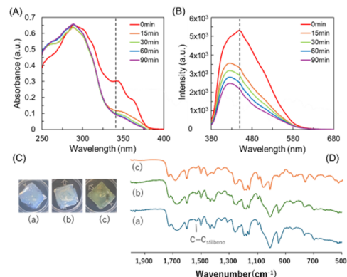
Fig. 5 (A) UV spectra of the prepared gel after UV irradiation for different times. (B) Fluorescence spectra of the prepared gel after UV irradiation at 256 nm. (C) Photograph and (D) IR spectra of the prepared gel (a) before and after UV irradiation at (b) 365 nm and (c) 256 nm.
