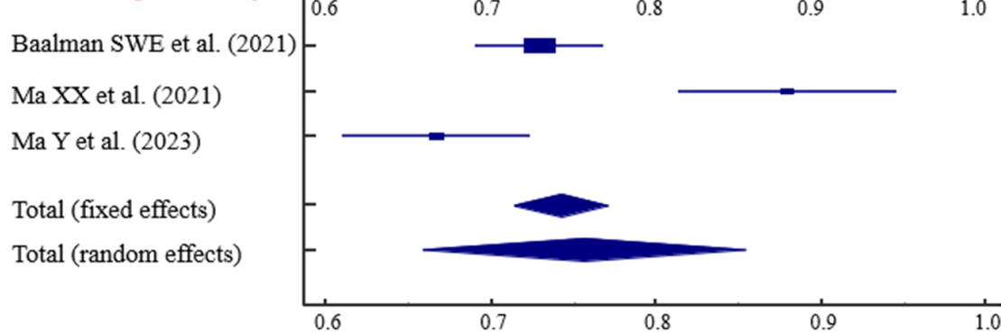
Figure 4. Subgroup analysis of follow-up time.
