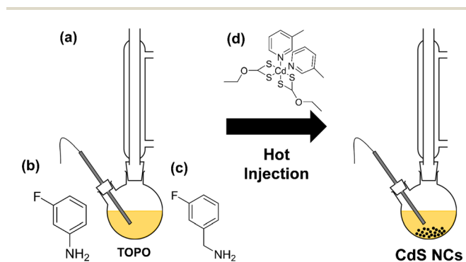
Fig. 1 (a) Reaction scheme of the hot injection method to form colloidal CdS nanocrystals. Also shown are the chemical structures of (b) 3-FLAn, (c) 3-FLBzAm and (d) [\text{Cd}(\text{Xan})_2(3\text{mpy})_2] .
