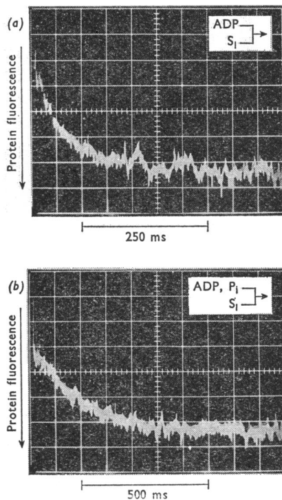
Fig. 7. Stopped-flow spectrophotometric record of the protein fluorescence during the reaction of ADP with subfragment 1 in the presence of P_i
