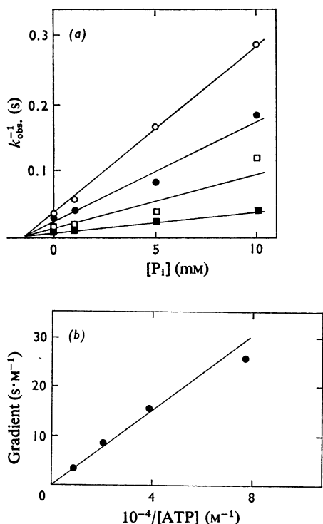
Fig. 6. Plot of P_i inhibition data to determine K_{P_i}
