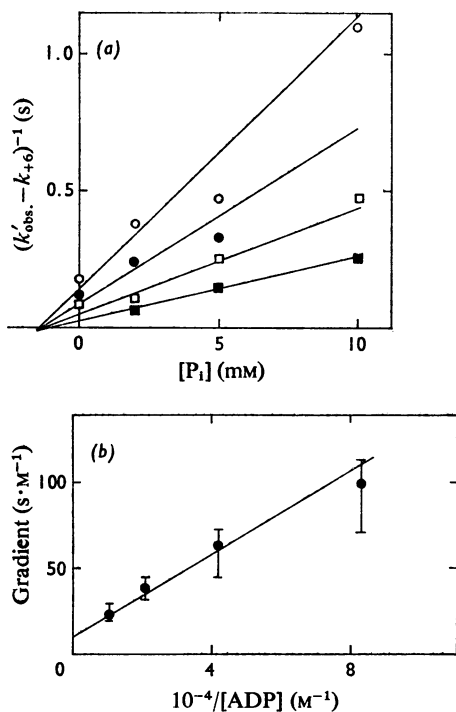
Fig. 9. Inhibition of ADP binding by P_i
