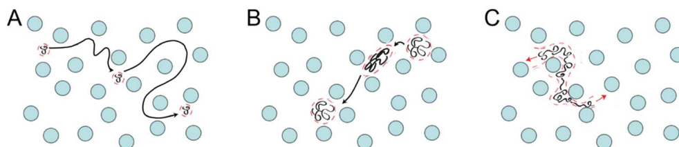
Fig. 4 DNA separation process utilizing gel electrophoresis. (A) R_g/a \ll 1 . (B) R_g/a \approx 1 (C) R_g/a \gg 1 .
