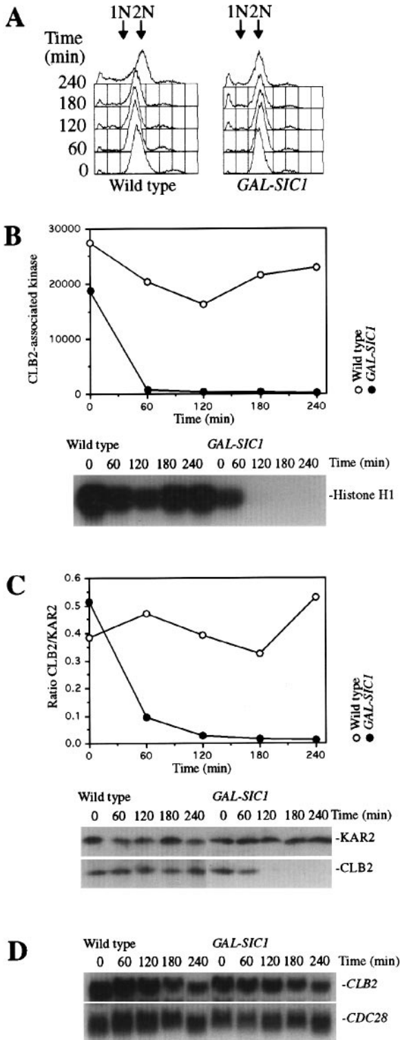
Fig. 3. Post-transcriptional mechanisms are responsible for Clb2 decay induced by inactivation of Cln- and Clb-dependent kinases. Cells deleted for CLB2 carrying CLB2 under the control of the constitutive S.pombe ADH promoter (A724; MATa , clb2::LEU2 , ADH-CLB2::URA3 ; ○) or an ADH-CLB2 strain carrying five copies of GAL-SIC1 (A725; MATa , clb2::LEU2 , ADH-CLB2::URA3 , 5x GAL-SIC1::TRP1 ; ●) were grown and arrested as described in the legend to Figure 2. After galactose and \alpha -factor addition, cell samples from indicated times points were analyzed for DNA content (A), Clb2-associated kinase activity (B), Clb2 protein (C) and CLB2 RNA (D).
