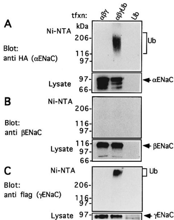
Fig. 2. Ubiquitination of \alpha and \gamma , but not \beta , ENaC expressed in Hek-293 cells. Hek-293 cells transiently co-transfected (txfn) with HA-tagged \alpha ENaC ( \alpha ), FLAG-tagged \gamma ENaC ( \gamma ), \beta ENaC ( \beta ) and/or the His-Ub (Ub) construct were lysed and lysates incubated with \text{Ni}^{2+} -NTA agarose beads ( \text{Ni}^{2+} -NTA) to precipitate histidinated (ubiquitinated) proteins. These proteins were separated on 7% SDS-PAGE, transferred to nitrocellulose and blotted with (A) anti-HA antibodies (to detect ubiquitinated \alpha ENaC), (B) anti- \beta ENaC antibodies (to detect ubiquitinated \beta ENaC) and (C) anti-FLAG (flag) antibodies (to detect ubiquitinated \gamma ENaC). Ubiquitinated species appear as a cluster of high molecular weight bands (upper panels, square brackets). Lower panels of each blot (Lysate) represent expression of the transfected protein ( \alpha -, \beta - or \gamma ENaC) in the lysates. Arrows indicate fully glycosylated forms of ENaC subunits.
