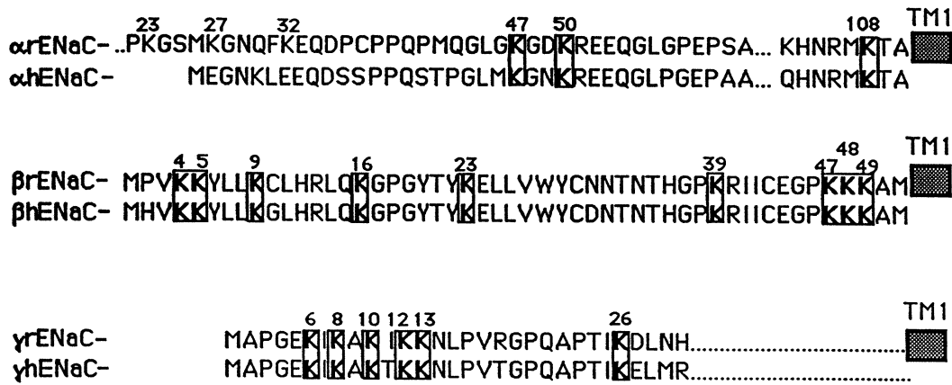
Fig. 3. N-terminal Lys to Arg mutants of \alpha\beta\gamma ENaC. Schematic representation of the conserved lysine residues at the N-termini of \alpha\beta\gamma rENaC and \alpha\beta\gamma hENaC. All conserved lysines (Bold letters, boxed), as well as three non-conserved lysine residues in \alpha ENaC, are numbered according to the published rat ENaC sequences (Canessa et al. , 1994a). The numbered lysines were mutated to arginines to create the following mutant constructs: in \alpha ENaC: \alpha K47,50R, \alpha K108R, \alpha K47,50,108R and \alpha K23-50R; in \beta ENaC: \beta K4,5,9R and \beta K16-49R; in \gamma ENaC: \gamma K6-13R, \gamma K26R and \gamma K6-13R + K26R. (TM1 = the first transmembrane domain of each ENaC subunit.)
