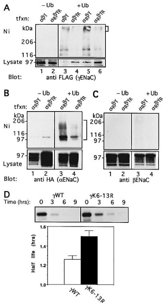
Fig. 6. Inhibition of ubiquitination of the Lys to Arg mutants of \gamma - and \alpha\text{ENaC} . Hek-293 cells were transiently co-transfected (tfxn) with \beta\text{ENaC} ( \beta ), HA-tagged \alpha\text{ENaC} ( \alpha ) or \alpha\text{K23-50R} ( \alpha\text{R} ), and FLAG-tagged \gamma\text{ENaC} ( \gamma ) or \gamma\text{K6-13R} ( \gamma\text{R} ), with or without His-Ub (Ub). Cells were then lysed, and lysates incubated with \text{Ni}^{2+} -NTA agarose beads to precipitate ubiquitinated proteins. Precipitated proteins were separated on 7% SDS-PAGE, transferred to nitrocellulose and blotted with either (A) anti-FLAG ( \gamma\text{ENaC} ), (B) anti-HA ( \alpha\text{ENaC} ) or (C) anti- \beta\text{ENaC} antibodies (upper panels), to detect ubiquitination of each subunit or its Lys to Arg mutants in the same experiment. Lower panels represent levels of expression of the transfected proteins in the lysate. Square brackets mark the ubiquitinated species of \alpha and \gamma ENaC. The ~105 kDa band across panel B (top) is probably a contaminant. (D) \gamma\text{K6-13R} mutant is more stable than wt- \gamma\text{ENaC} . MDCK cells stably expressing wt- \alpha\beta\gamma\text{ENaC} (called \gamma\text{WT} ) or \gamma\text{K6-13R} plus wt- \alpha\beta\text{ENaC} (called \gamma\text{K6-13R} ) (both \gamma subunits FLAG-tagged at the C terminus, as in Figure 2 above) were labelled with [ ^{35}\text{S} ]Met/Cys and chased for the indicated times (hrs). Cells were then lysed, immunoprecipitated with anti \gamma\text{ENaC} antibodies, the immunoprecipitates separated on 7% SDS-PAGE and visualized by autoradiography, as represented by the autoradiogram. Histogram represents t_{1/2} quantitation (mean \pm SE) of three independent experiments similar to that depicted in the autoradiogram.
