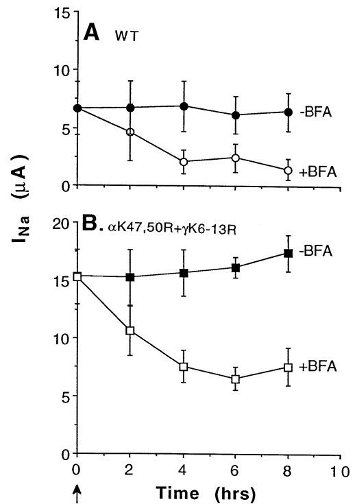
Fig. 7. The effect of Brefeldin A on channel activity of wt-ENaC or the \alpha\text{K47,50R}+\gamma\text{K6-13R} mutant. cRNA from (A) wt- \alpha\beta\gamma\text{ENaC} (WT) or (B) the \alpha\text{K47,50R}+\gamma\text{K6-13R} (plus wt- \beta ) mutant, was injected into Xenopus oocytes. Eighteen hours later, 10 \mu\text{g/ml} Brefeldin A (BFA) were added (at time 0, arrow) to the bathing medium and amiloride-sensitive \text{Na}^+ currents ( I_{\text{Na}} ) measured by the two-electrode voltage clamp technique at the indicated times. Data points represent mean \pm SE of four separate experiments each performed with five oocytes.
