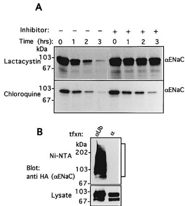
Fig. 9. Ubiquitination and mode of degradation of \alpha ENaC expressed alone in MDCK cells. (A) HA-tagged \alpha ENaC stably expressed in MDCK cells was labelled with ^{35}\text{S} Met and Cys for 2 h, and chased for the indicated times in the absence (–) or presence (+) of 10 \mu\text{M} lactacystin added during the pulse and the chase periods (upper panel), or 0.4 mM chloroquine added during the chase period (lower panel), as described in Figure 8 above. (B) Ubiquitination of \alpha ENaC transfected with His-Ub (Ub) into Hek-293 cells. Histidinated (ubiquitinated) proteins were precipitated on Ni-NTA agarose beads, proteins separated on 7% SDS-PAGE and immunoblotted with anti-HA antibodies, to detect ubiquitinated species of \alpha ENaC. The square bracket depicts ubiquitinated \alpha ENaC. The control ( \alpha , right lane) was transfected with \alpha ENaC without His-Ub, and reveals no detectable ubiquitination, similar to cells transfected with \alpha ENaC alone.
