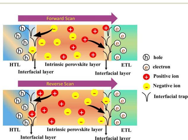
Fig. 7 Schematic diagram shows the different ions movements in perovskite device structure during forward and reverse scan, which can lead the hysteresis phenomenon and degrade the device stability as well as performance. Figure reproduced with permission from ref. 9.
