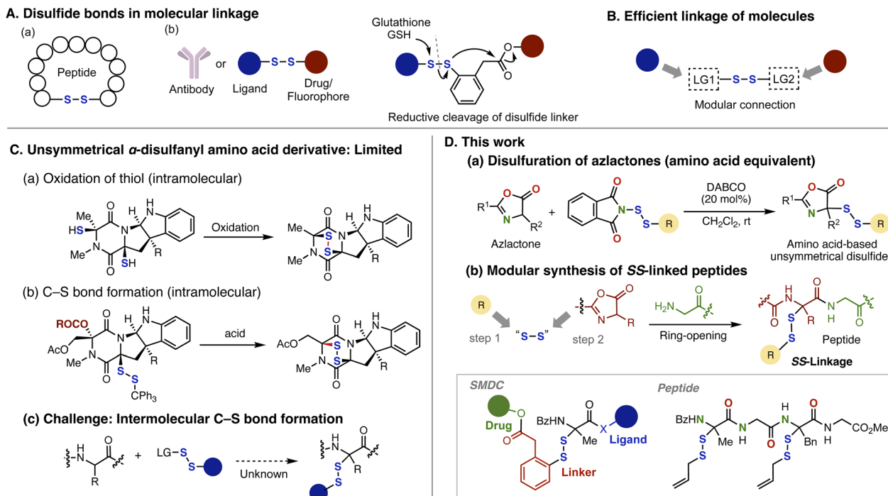
Fig. 1 Preparation of amino acid/peptide-based disulfides. (A) Disulfide bonds in molecular linkage. (B) Ideal synthetic method for efficiently linking peptides. (C) Synthetic method for the preparation of \alpha -disulfurated amino acid derivatives. (D) This work: modular preparation of SS-linked peptides through disulfuration reaction of azlactones. SMDC: small molecule–drug conjugates.
