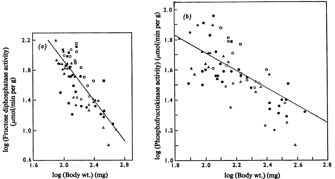
Fig. 1. Enzyme activities in bumble-bee flight muscle as a function of body weight
