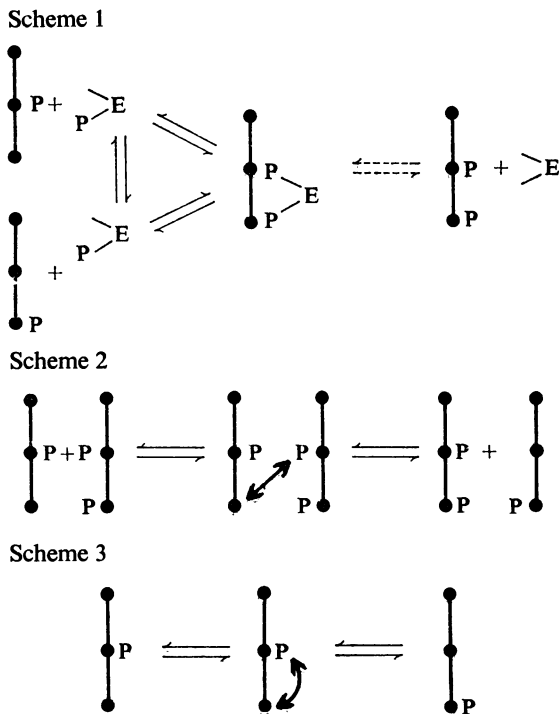
Fig. 1. Possible schemes for the phosphoglycerate mutase reaction
