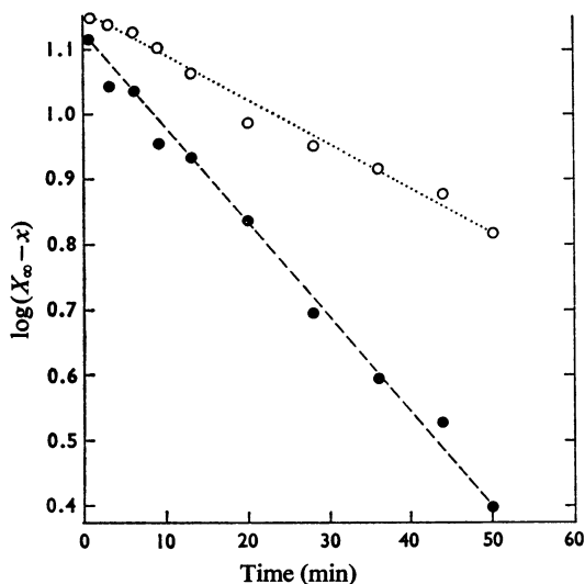
Fig. 6. Measurement of fluxes at equilibrium
