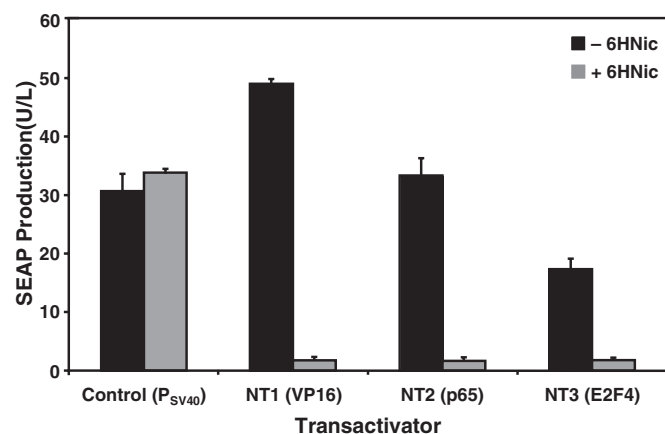
Figure 4. Regulation performance of different 6HNic-dependent transactivators. A. nicotinovorans pAO1's 6HNic oxidase repressor HdnoR was fused to different transactivation domains derived from (i) H. simplex virus (VP16; NT1, HdnoR-VP16), (ii) human NF- \kappa B (p65; NT2, HdnoR-p65) and (iii) human E2F4 (E2F4; NT3, HdnoR-E2F4). The regulation performance of NT1, NT2 and NT3 was assessed by cotransfection of either pLM82 ( P_{SV40} -NT1-pA), pLM101 ( P_{SV40} -NT2-pA) or pLM102 ( P_{SV40} -NT3-pA) and pLM104 ( P_{NIC1b} -SEAP-pA) into CHO-K1 followed by cultivation for 48 h in the presence and absence of 6HNic and SEAP quantification. SEAP production was compared with pSEAP2-Control-transfected CHO-K1 cells harboring a glycoprotein expression unit driven by the constitutive SV40 promoter ( P_{SV40} ).
