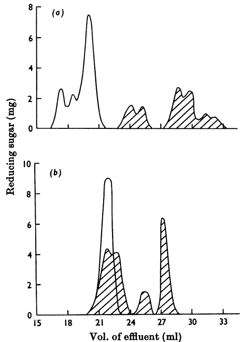
Fig. 6. Mobility of cationic and anionic glycopeptides on Sephadex G-10 after proteolytic digestion. Fractions P7.50a (a) and P7.1a (b) were chromatographed on columns (1 cm × 55 cm) and the material indicated under the non-hatched curves was digested with Pronase and subtilisin. The digests were rechromatographed on the same columns. The hatched areas represent amounts of reducing sugar after proteolysis.
