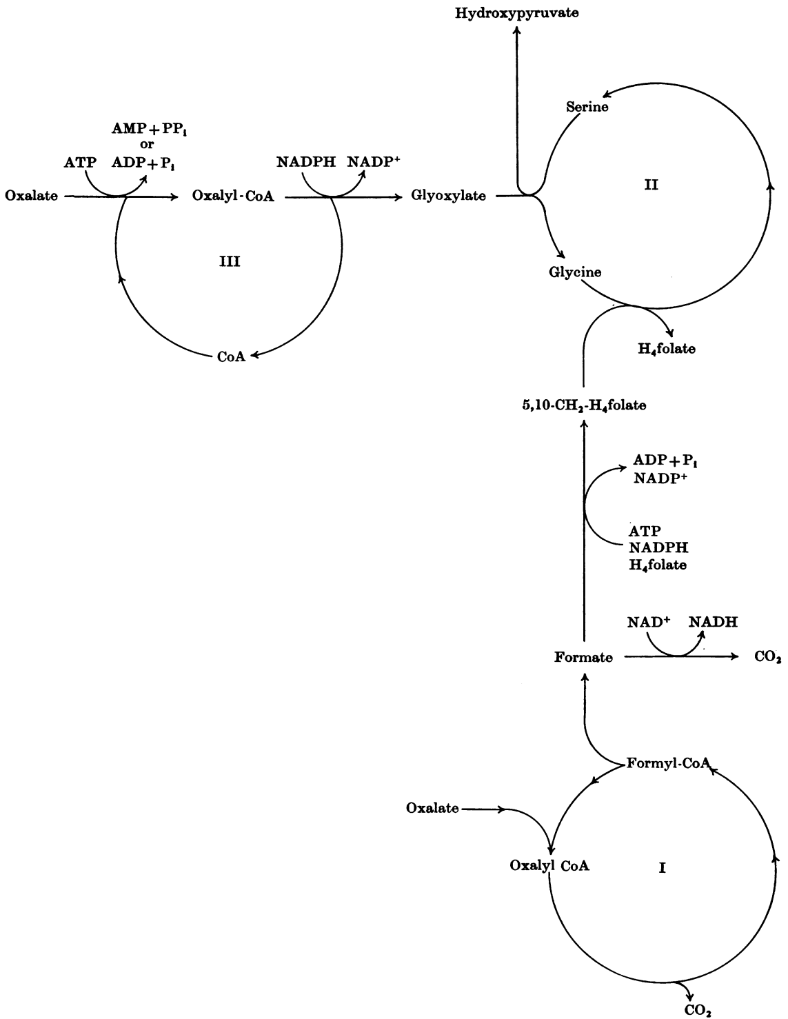
Scheme 1. Conversion of oxalate into hydroxypyruvate.
