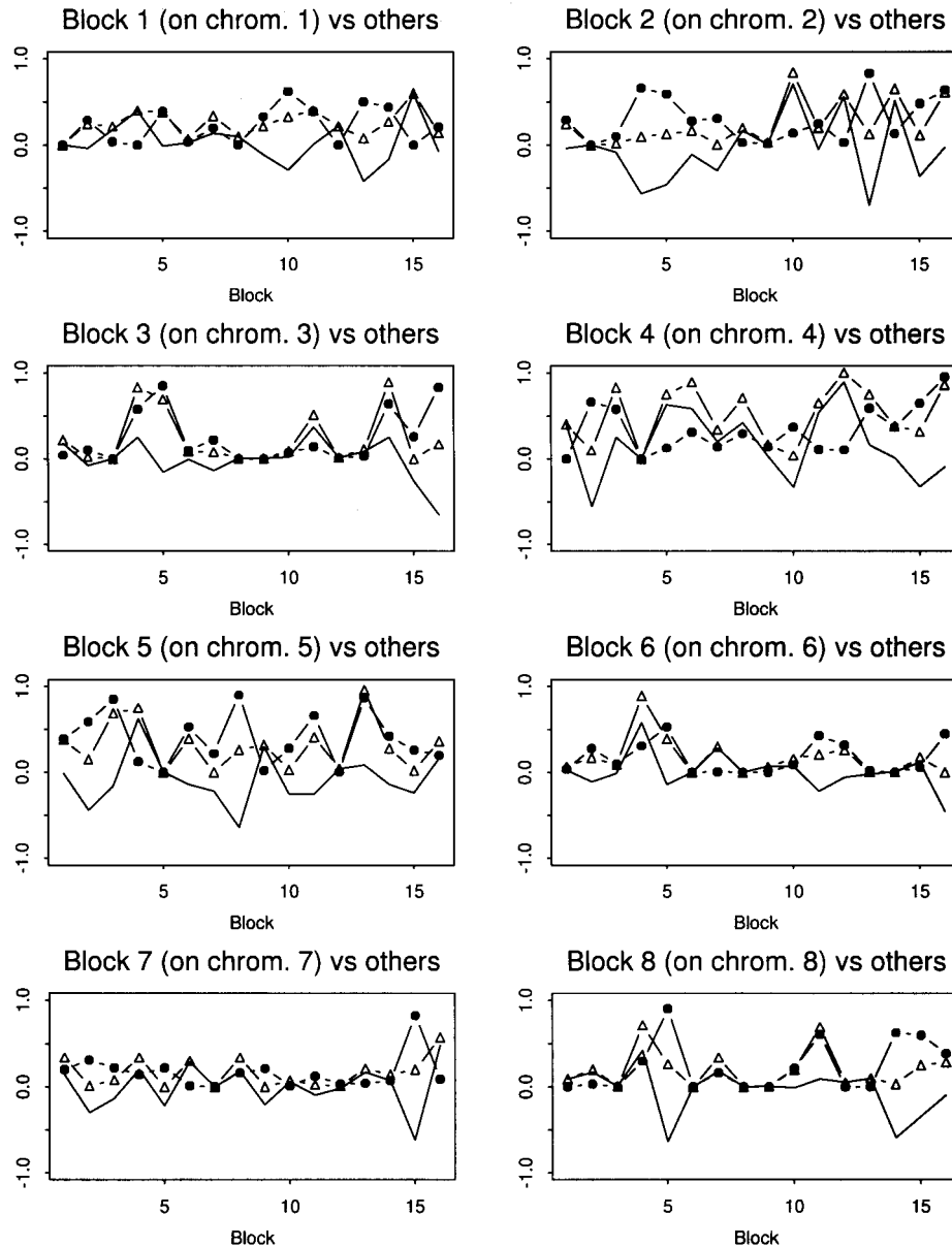
Figure 2 The P values of testing the interactions of blocks 1–8 with the other blocks, for the cases and controls in the Dutch type 1 diabetes data. The dotted lines are for the cases, and the lines with small triangles are for the controls. The normal line, a contrast between the two lines, is derived by subtracting the corresponding P values of the control from those of the case.
