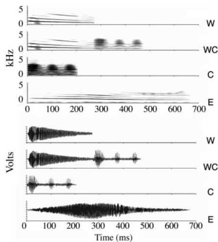
Fig. 1. Recordings of natural mating calls used as acoustic stimuli. Sonograms ( Upper ) and waveforms ( Lower ) of acoustic stimuli broadcast to frogs. Top to bottom for each: P. pustulosus whine, P. pustulosus whine–chuck, chuck-only, and heterospecific P. enesefae whine.
