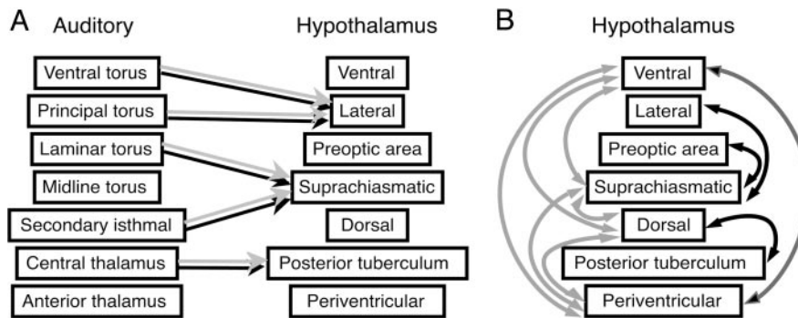
Fig. 5. Functional connectivity of the hypothalamus. Gray arrows show significant relationships ( P < 0.05 ) in frogs that heard irrelevant acoustic stimuli ( P. enesefae whine and chuck-only), and black arrows indicate relationships in frogs exposed to behaviorally relevant stimuli (conspecific whine and whine–chuck). (A) egr-1 levels in midbrain and thalamic nuclei implicated in auditory processing are significant predictors of hypothalamic expression patterns. Relationships between auditory and hypothalamic regions do not vary with relevance of stimulus. (B) egr-1 correlations between hypothalamic regions differ based on behavioral relevance of acoustic stimulus.
