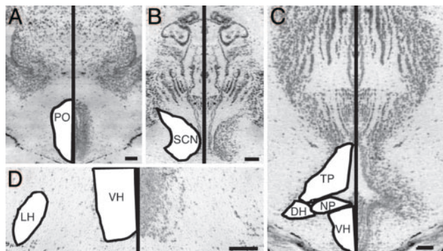
Fig. 2. Photomicrographs of cresyl-violet-stained transverse sections through frog brain. Left half of photographs are mirror images of right half for clarity. Hypothalamic nuclei are labeled on figures based on standard nomenclature (31) with the following abbreviations: DH, dorsal hypothalamus; NP, nucleus of the periventricular organ; POA, anterior POA; VH, ventral hypothalamus. (Bar, 100 \mu\text{m} .) ( A ) The second-most rostral section we used for POA analysis. ( B ) Section containing the SCN comparable to figure 3 A in ref. 31. ( C ) Third-most rostral section containing the infundibular hypothalamus, equivalent to figure 5 A in ref. 31. ( D ) Higher-magnification image showing sparse cells in the LH at a level corresponding to figure 4 A of ref. 31.
