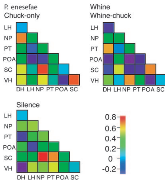
Fig. 4. Pair-wise correlations between hypothalamic nuclei vary with acoustic stimulus. Pair-wise Pearson correlation coefficients between nuclei calculated for unstimulated animals, for animals hearing irrelevant calls (chuck-only and P. enesefae whine), and for frogs exposed to behaviorally relevant calls (conspecific whine and whine–chuck). Coefficient coded by color scale (Lower Right) with red colors representing high and blue indicating low coefficients.
