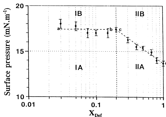
FIGURE 3 Transition pressure-composition diagram for mixed defensin A/lecithin monolayers. The dotted line ab is drawn according to \pi_t = 17.4 \pm 0.4 \text{ mN} \cdot \text{m}^{-1} ; the dotted line cd is drawn according to \pi_t = 13.7 - 2.3 \ln X_{\text{Def}} . IA region: Lecithin in the LE state, defensin-lecithin 1/4 complex in the LE state (not miscible with the excess lecithin). IB region: Lecithin in the LE state, defensin-lecithin complex in a condensed state. IIA region: Defensin-lecithin complex in the LE state (miscible with the excess defensin). IIB region: Defensin and the complex in a condensed state (miscible).
