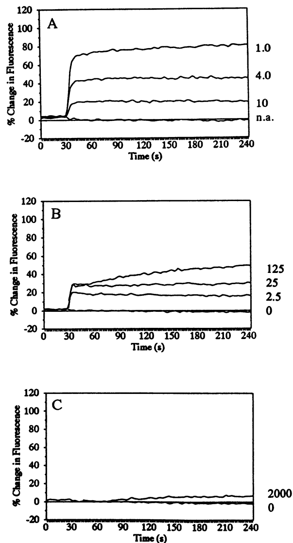
FIGURE 5 Effect of (A) pCMV5 plasmid, (B) citrate, and (C) NaCl on fusion of DOTMA/DOPC (1:1) vesicles in 20 mM HEPES (pH 7.4) at 25 ^{\circ}\text{C} . Vesicles were prepared with and without 0.5 mol% each of NBD-PE and Rh-PE. The labeled and unlabeled vesicles were mixed in a 1:9 ratio and diluted to 0.50 mM total lipid. Different anions were added at 30 s. The concentration of citrate and NaCl (mM), and the charge ratio of DNA-cationic lipid complexes are indicated. The system without pCMV5 is indicated by “n.a.” The charge ratio is defined as moles of DOTMA/moles of phosphorus in pCMV5.
