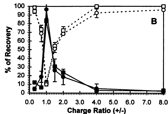
FIGURE 10 DNA and lipid recovery in supernatant and pellet fractions after centrifugation of DNA-cationic lipid complexes. Trace amounts of ^3\text{H} pCMV \beta gal and ^{14}\text{C} CHOL-HEX, and 20 \mu\text{g} pCMV \beta gal were used for both pCMV \beta gal-DOTMA/DOPE (A) and pCMV \beta gal-DOTMA/DOPC (B). DNA ( \circ , \bullet ) and lipid ( \square , \blacksquare ) recovery in the supernatant (---) and the resuspended pellet fractions (—) are shown. The charge ratio is defined as moles of DOTMA/moles of phosphorus in pCMV \beta gal.
