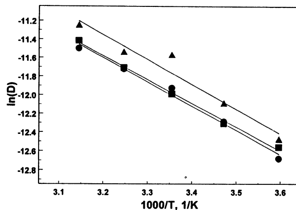
FIGURE 3 The temperature dependence of the derived translational diffusion constants for the headgroup TEMPO label (●), the 5-doxyl stearate label (■), and the 12-doxyl stearate label (▲) in POPC vesicles; pH values of 7.0, 8.0, and 8.0, respectively.
