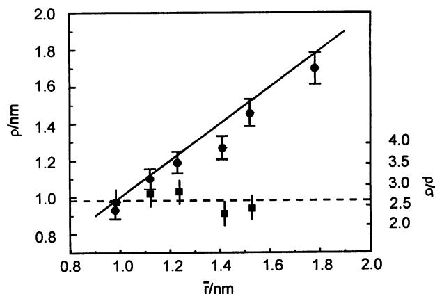
FIGURE 7 The fitted values of the interspin distance \rho (●) and of \rho/\sigma (■) for the samples shown in Fig. 6, b–g, plotted versus the average distance to the nearest nitroxide neighbor, \bar{r} , calculated from Eq. 7. The full line shows the function \bar{r} = \rho , and the dashed line is the average value of \rho/\sigma = 2.6 . For interspin values exceeding 1.8 nm no reasonable values for \sigma could be fitted due to the very small dipolar broadening of the spectra. In this case \sigma was fixed to \rho/2.64 .
