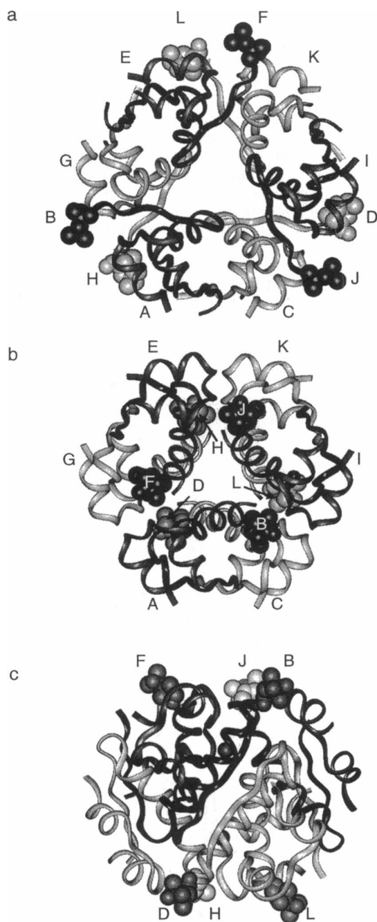
FIGURE 2 The B2SL insulin hexamer ( a ) in the T6 state and ( b ) in the R6 state as seen along the three-fold axis. The strands show the peptide backbone of the chains labeled A through L; the spin labels attached to the B-chains labeled B, D, F, H, J, and L are plotted space filled. The Zn ions and the phenols that stabilize the R6 structure are omitted. The electron spin probes are seen on the hexamer surface organized as two sets of trimers. For the T6 state, the respective spin probe positions were modeled; x-ray data of the spin labeled hexamers reveal the structure of the R6 state. The three poorly defined spin probe moieties were generated by symmetry operation from their well defined equivalents. After this operation, the generated coordinates were seen to sit sensibly in the low-level electron density. ( c ) A view of the B2SL insulin hexamer in the R6 state with the three-fold axis vertical. Here, the Zn ions are shown as spheres; they lie on the three-fold axis and are \sim 1.5 nm apart.
