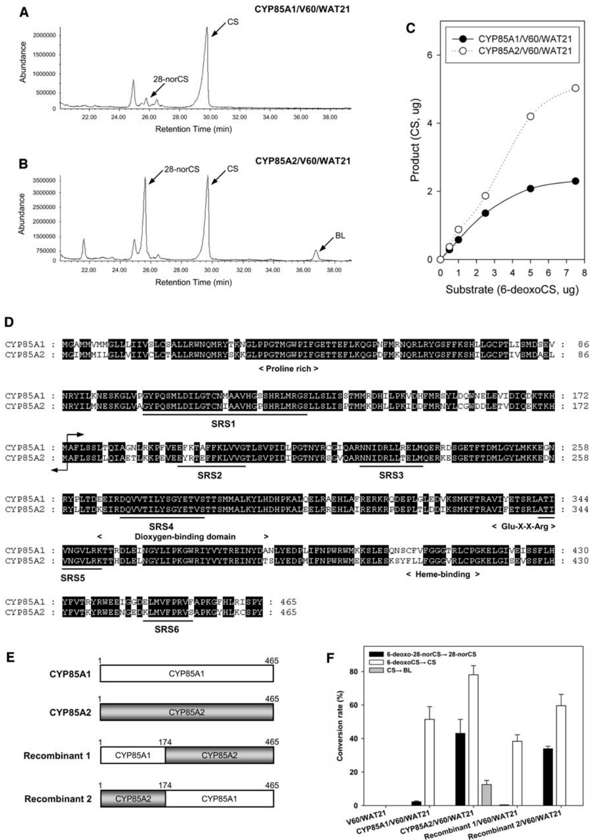
Figure 2. Biochemical Analysis of CYP85A1 and CYP85A2 Enzyme Activity.
