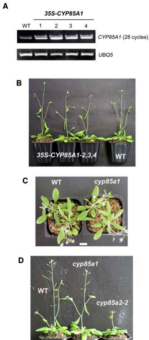
Figure 6. Phenotype of CYP85A1 Overexpression and cyp85a1 Mutant.
