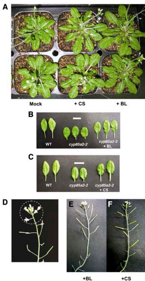
Figure 4. Rescue of Abnormalities in the cyp85a2 Mutant by Application of CS and BL.
