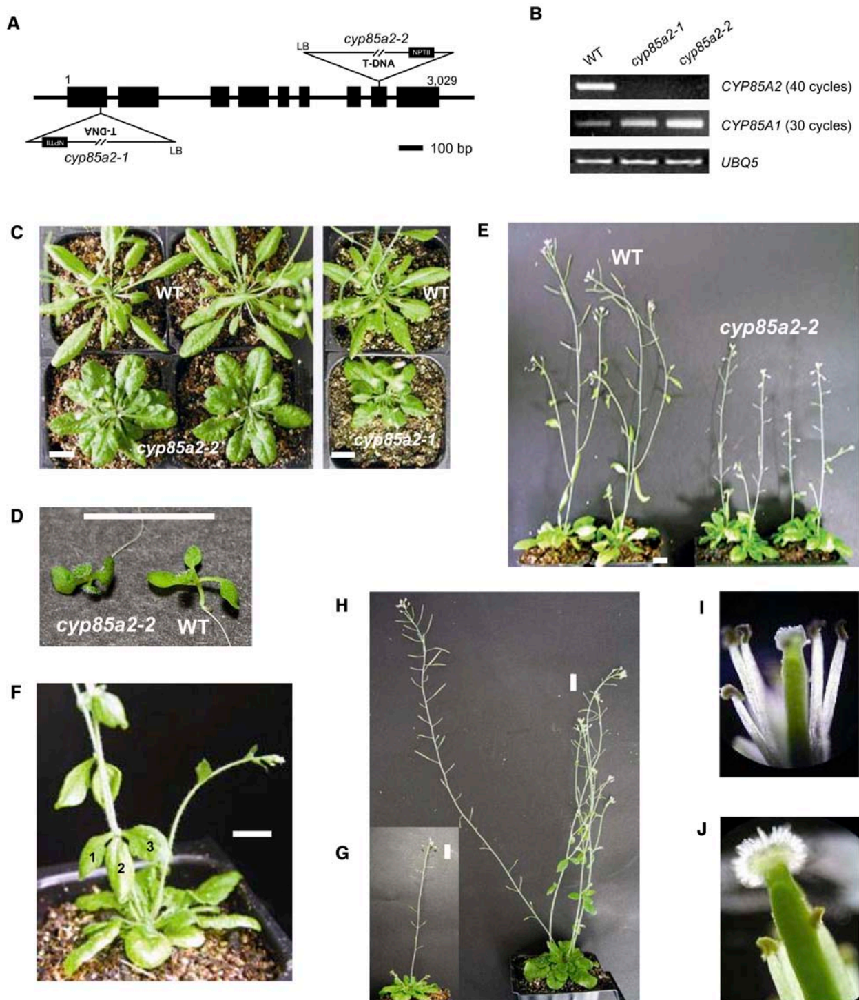
Figure 3. Phenotype of Arabidopsis CYP85A2 -Deficient Mutants cyp85a2-1 and cyp85a2-2 .
