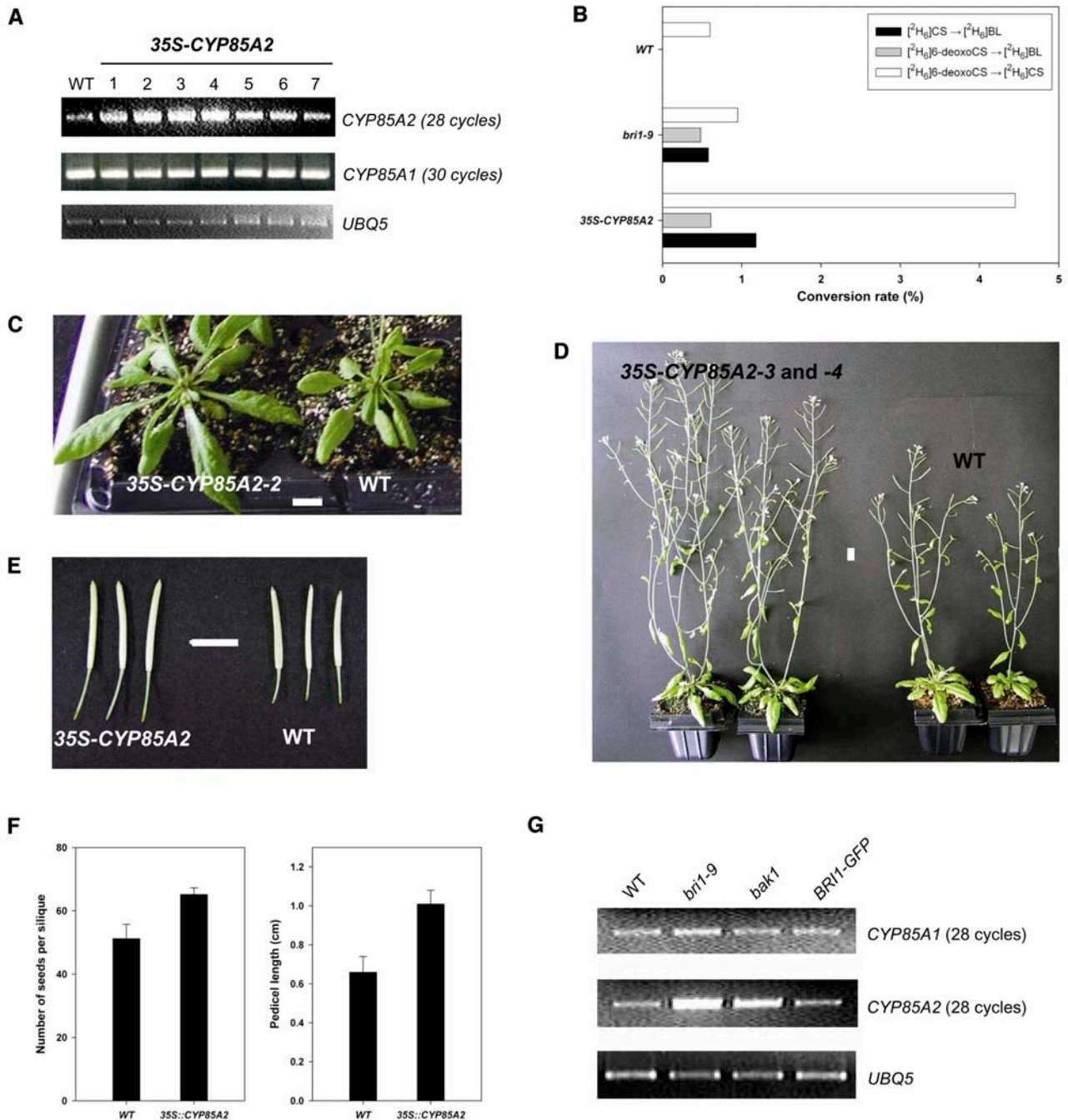
Figure 5. Biochemical Analysis and Phenotype of Arabidopsis CYP85A2 Overexpression Plants, 35S-CYP85A2.
