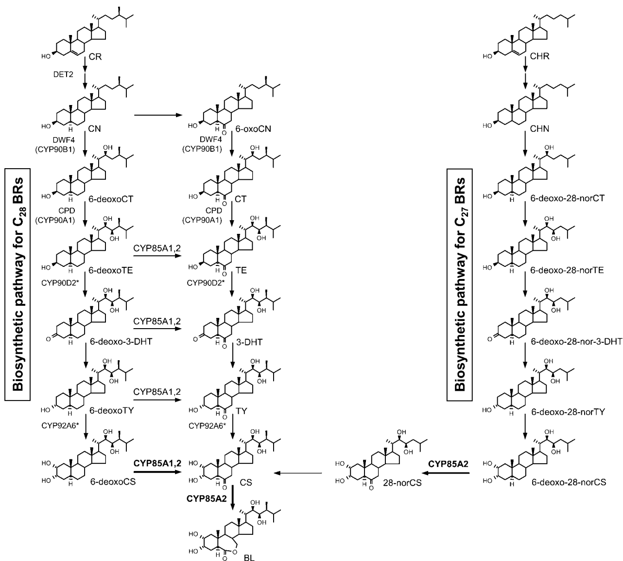
Figure 1. Biosynthetic Pathways to Generate BL in Plants.
