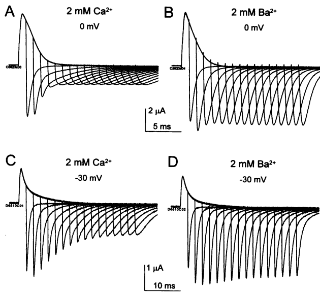
FIGURE 5 Influence of Ba 2+ on Q_{OFF} is time-dependent. Gating currents evoked with either 2 mM Ca 2+ (A and C) or 2 mM Ba 2+ (B and D) in the external solution. The membrane was stepped from -90 mV to 0 mV (A and B) or -30 mV (C and D) and then repolarized to -90 mV; depolarizing durations were in increments of 1 and 2 ms, respectively. (A) and (B) were from the same oocyte and (C) and (D) were from the same oocyte.
