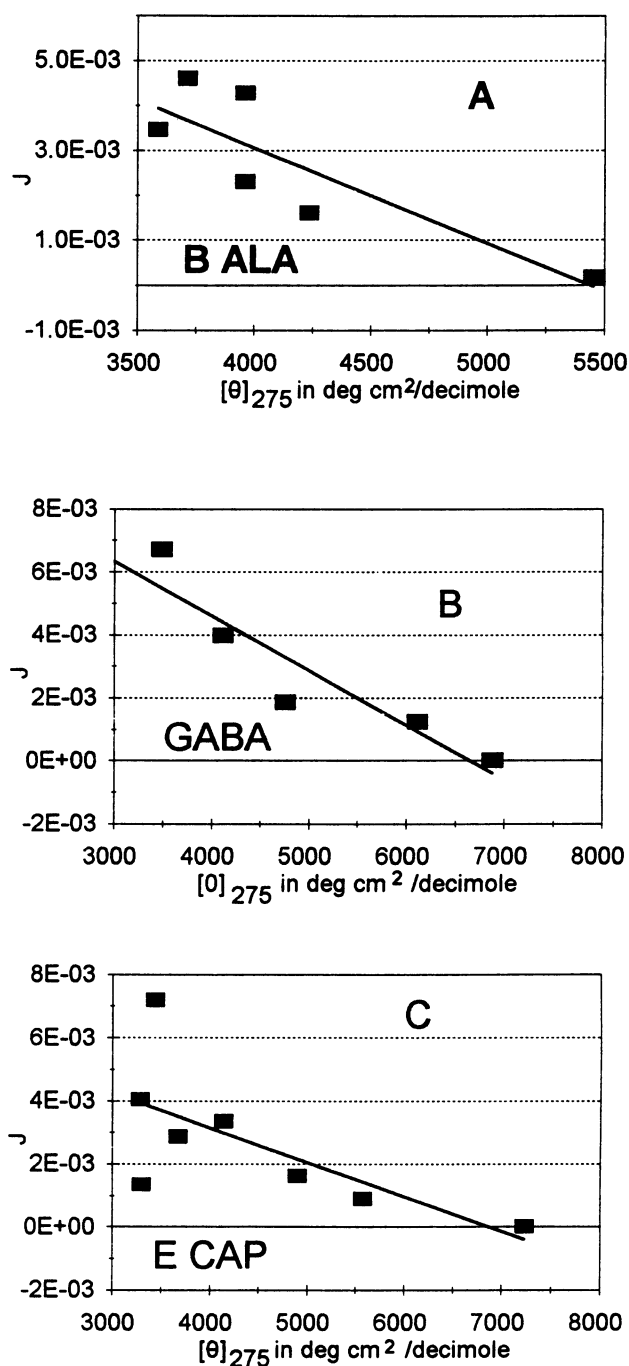
FIGURE 7 Plots of the J function, defined in Eq. 9, against [\theta]_{275} . (A) B ALA, (B) GABA, and (C) E CAP.
