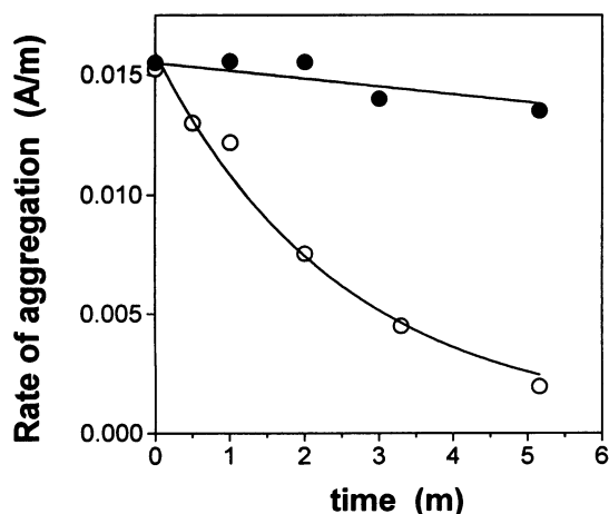
FIGURE 5 Effect of membrane binding on the rate of reduction with dithiothreitol. Annexin I (1.5 \mu\text{g/ml} ) was bound to 10 \mu\text{M} PS (○). Dithiothreitol (5 mM) was added, and aggregation was started at the specified times with 1 mM \text{CaCl}_2 . For the experiments with free annexin I (●), DTT was incubated with annexin I, and PS and 1 mM \text{CaCl}_2 were added at the specified times to start aggregation. Curves were drawn by eye.
