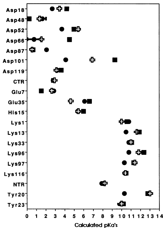
FIGURE 3 pK_a 's calculated by the multiconformation ( \oplus ) and fixed structure methods ( \blacksquare ), and the experimental data ( \bullet ) (Karamitsu and Hamaguchi, 1980; Bartik et al., 1994) (Tyr53 is not included). Error bars reported for the measurements of Bartik et al. (1994), which are used for acidic pH (Glu, Asp, and His) pK_a 's. Data from Kuramitsu and Hamaguchi (1980) were used for all other residues. Arg is not shown.
