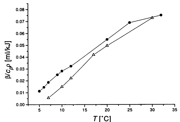
FIGURE 2 Temperature dependence of \beta/c_p\rho (●) for a Ringer's solution in the presence of washed membranes, \lambda_{\text{exc}} = 650 nm, and (Δ) for a Ringer's solution containing 2% dodecyl- \beta -D-maltoside and bleached rhodopsin, \lambda_{\text{exc}} = 500 nm. In both cases Evans blue served as a calorimetric reference. A relatively large integration time of \sim 1.5 \mu\text{s} was used.
