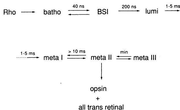
FIGURE 1 Simplified reaction scheme describing the events in the first microseconds following excitation of rhodopsin. Modified after Hofmann (1995) and Kligler and Lewis (1995). The time constants of 40 and 200 ns are the apparent decay times of batho and BSI at ambient temperature in solubilized rhodopsin.
