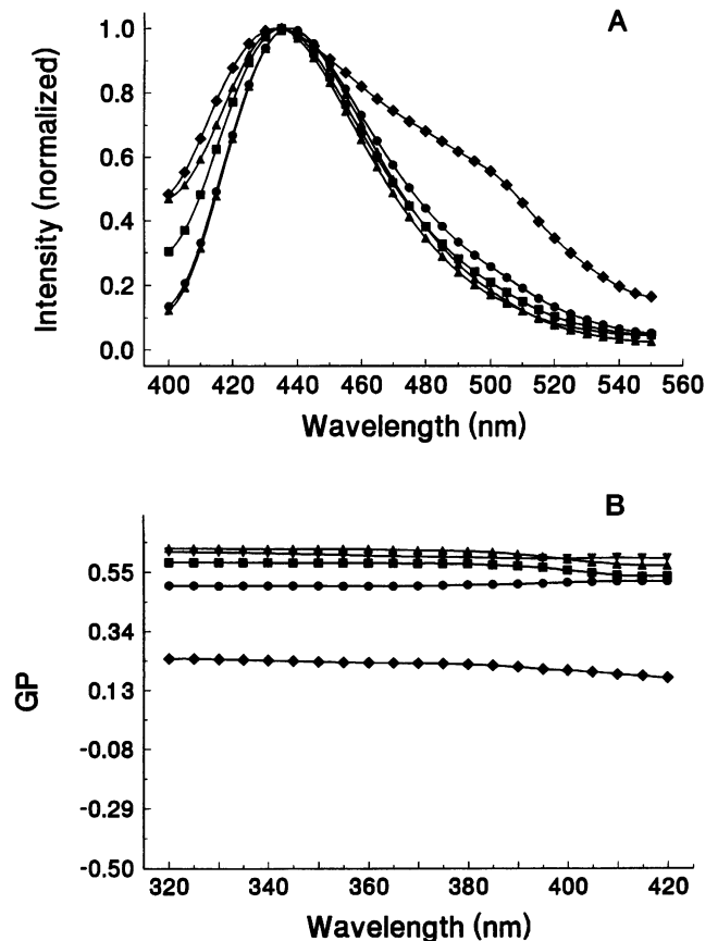
FIGURE 2 Normalized laurdan fluorescence emission spectra (A) and excitation GP spectra (B) in multilamellar phospholipid vesicles composed of 30 mol% cholesterol and DOPC ( \blacklozenge ), DLPC ( \bullet ), DPPC ( \blacktriangledown ) and of equimolar mixtures of DOPC and DPPC ( \blacktriangle ) and of DLPC and DPPC ( \blacksquare ) at 20°C.
