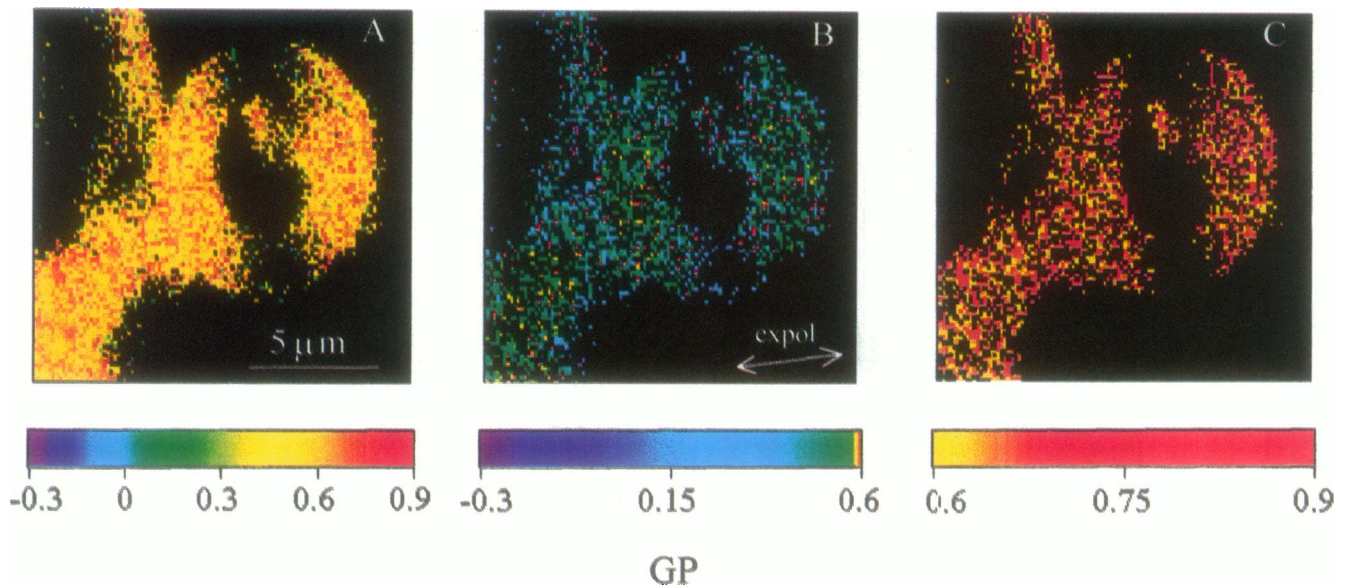
FIGURE 9 GP images of vesicles composed of DPPC and 30 mol% cholesterol labeled with laurdan at room temperature ( \sim 20^\circ\text{C} ). The colors indicate different GP values following the reported scale. The image scale bar is reported in A, together with the direction of the excitation polarization. In B and C only selected GP values are drawn, using the colors indicated in the corresponding scales. Polarized excitation light has been used; the direction of polarization is \sim 10^\circ with respect to the horizontal.
