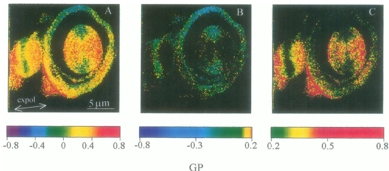
FIGURE 7 GP images of vesicles composed of the equimolar mixture of DOPC and DPPC labeled with laurdan at room temperature ( \sim 20^\circ\text{C} ). The colors indicate different GP values following the reported scale. The image scale bar is reported in A, together with the direction of the excitation polarization. In B and C only selected GP values are drawn, using the colors indicated in the corresponding scales. Polarized excitation light has been used; the direction of polarization is \sim 10^\circ with respect to the horizontal.
