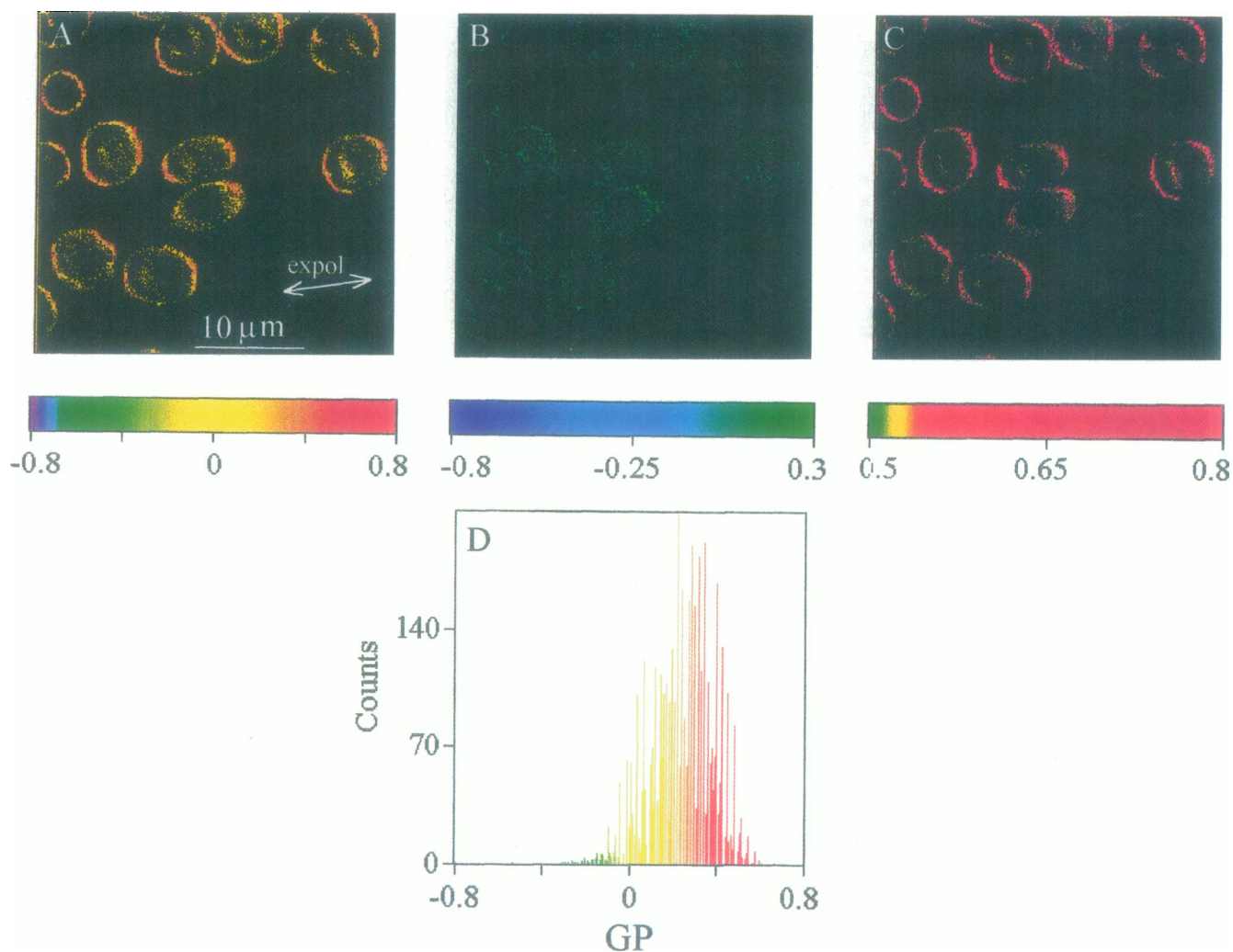
FIGURE 12 (A) GP images of red blood cells labeled with laurdan obtained at room temperature ( \sim 20^{\circ}\text{C} ). The colors indicate different GP values following the reported scale. In B and C the low and high GP values are drawn, respectively, following the reported scales. (D) Distribution of the GP values. The image scale bar is reported in A, together with the direction of the excitation polarization.
