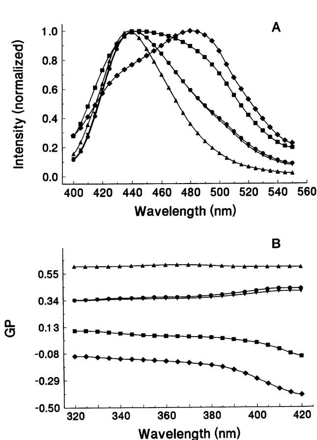
FIGURE 1 Normalized laurdan fluorescence emission spectra (A) and excitation GP spectra (B) in multilamellar phospholipid vesicles composed of DOPC ( \blacklozenge ), DLPC ( \blacksquare ), and DPPC ( \blacktriangle ) and of equimolar mixtures of DOPC and DPPC ( \blacktriangledown ) and of DLPC and DPPC ( \bullet ) at 20°C.
