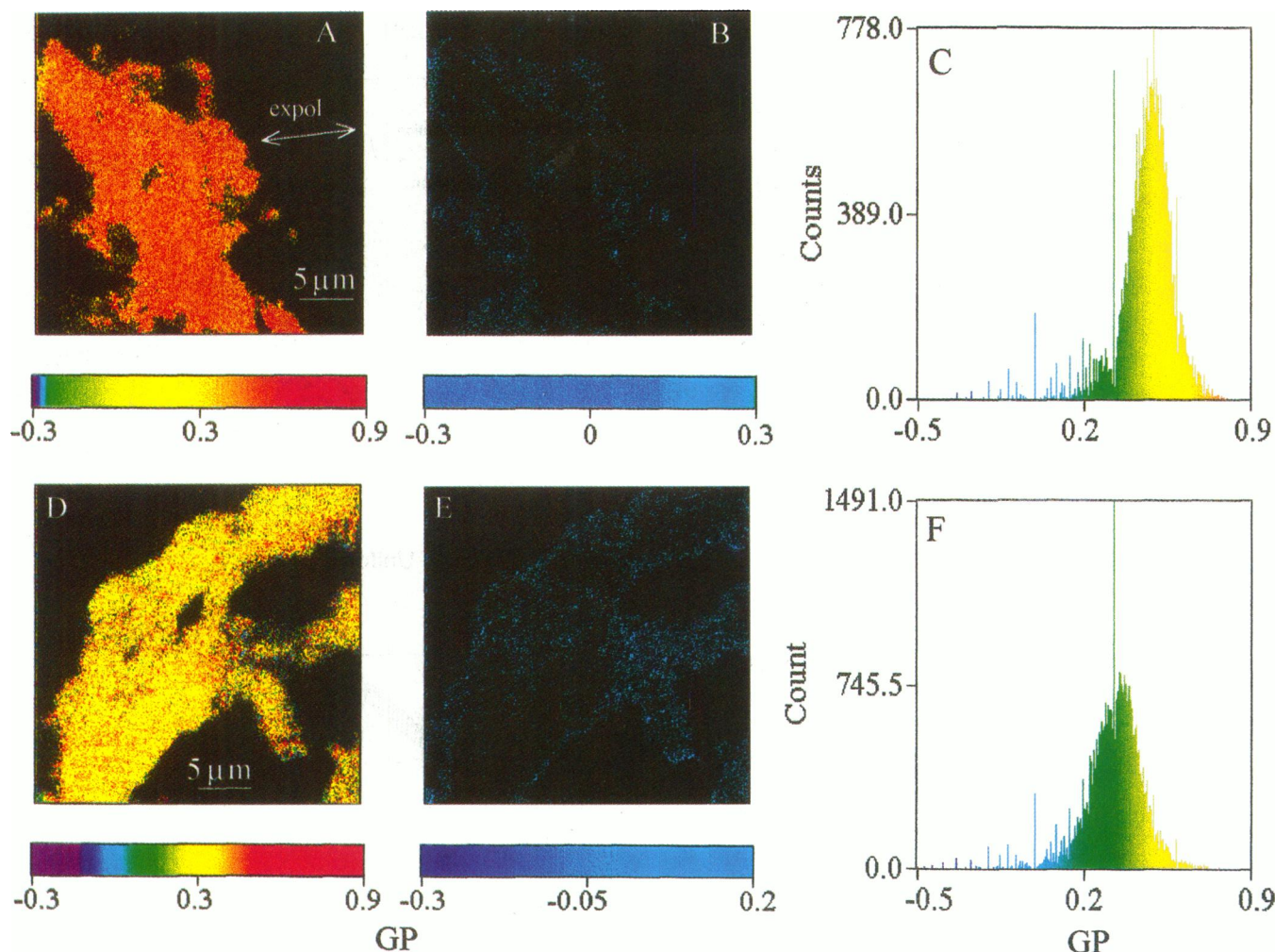
FIGURE 15 GP images ( A , B , D and E ) and histograms ( C and F ) of purified rat renal brush border ( A , B , and C ) and basolateral membranes ( D , E , and F ) labeled with laurdan at room temperature ( \sim 20^{\circ}\text{C} ). The colors indicate different GP values following the reported scales. The image scale bar is reported in A , together with the direction of the excitation polarization. In B and E only low GP values are drawn, using the colors indicated in the corresponding scales. Polarized excitation light has been used; the direction of polarization is \sim 10^{\circ} with respect to the horizontal.
