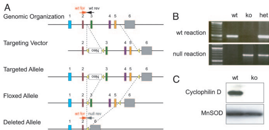
Fig. 1. Deletion of CypD. (A) Schematic of the CypD locus. PCR primers distinguishing WT and null alleles are designated. wt for, WT forward; wt rev, WT reverse; null rev, null reverse. (B) Genotyping of CypD WT/WT using WT forward and WT reverse primers generated a 490-bp product in the WT allele. Genotyping of CypD null/null mice using the null primer set WT forward and null reverse generated a 700-bp product. (C) Western blots of mitochondria purified from CypD WT/WT and CypD null/null mice using a CypD-specific antibody.
