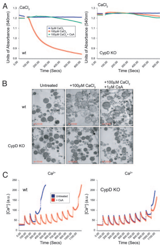
Fig. 2. Induction of PT in CypD-deficient and WT mitochondria. (A) Mitochondrial swelling induced by treatment with 100 \mu\text{M} \text{CaCl}_2 was measured by monitoring mitochondrial size at an absorbance of 540 nm. Mitochondria isolated from WT (Left) and CypD-deficient (Right) mice were resuspended at a concentration of 0.5 mg/ml in EB for 5 min. Where indicated (arrow), 100 \mu\text{M} \text{CaCl}_2 was added. Mitochondria were preincubated with 1 \mu\text{M} CsA or buffer alone for 5 min. (B) Transmission electron microscopy of liver mitochondria taken from WT and CypD-deficient mitochondria. Mitochondria were treated with 100 \mu\text{M} \text{CaCl}_2 for 200 s and fixed in 1.25% glutaraldehyde. (Scale bars, 200 nm.) (C) Loss of \text{CaCl}_2 buffering capacity in liver mitochondria isolated from WT and CypD-deficient mice resuspended at 0.5 mg/ml in EB. Extramitochondrial \text{Ca}^{2+} was measured fluorometrically with the calcium indicator Calcium Green 5N. Pulses of 10 \mu\text{M} \text{CaCl}_2 were added at intervals of 100 s.
