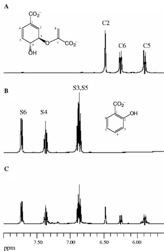
FIG. 3. ^1\text{H} NMR spectroscopic analysis of the Irp9-catalyzed conversion of chorismate to salicylate. Each spectrum was acquired at 27^\circ\text{C} over a period of 45 min in 20 mM potassium phosphate and 5 mM \text{MgCl}_2 , pH 7.0. (A) Substrate control, 2 mM chorismate. (B) Product control, 2 mM salicylate. (C) Irp9-catalyzed reaction, 10 \mu\text{M} Irp9 and 2 mM chorismate. Only the vinylic regions (5.0 to 8.0 ppm) of the NMR spectra are displayed. The abbreviations C and S correspond to protons from chorismate and salicylate, respectively.
