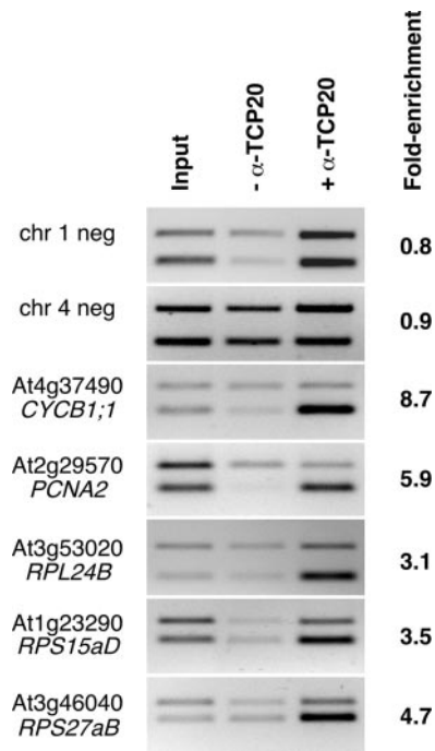
Fig. 6. p33^{TCP20} coregulates cell cycle and ribosomal protein genes. Chromatin cross-linked to DNA isolated from Arabidopsis seedlings was immunoprecipitated with anti- p33^{TCP20} antibodies. PCRs were performed with input DNA (Left), DNA precipitated without addition of anti- p33^{TCP20} antibodies (Center), and DNA immunoprecipitated with anti- p33^{TCP20} antibodies (Right). All reactions were performed in the presence of an internal control used to normalize reactions (top band), corresponding to sequences within At5g03545 (At4). Enrichment was calculated after normalizing input and immunoprecipitated reactions and comparing their ratios. Gene identifiers are shown at left.
